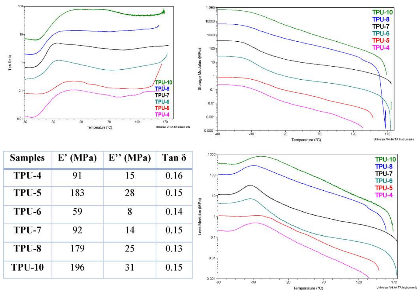
FIGURE 5 DMTA analyses of TPU-4 to TPU-10: \tan \delta (top left), storage modulus (top right), loss modulus (bottom right), and E' (storage modulus), and E'' (loss modulus) at 37°C [Color figure can be viewed at wileyonlinelibrary.com]
