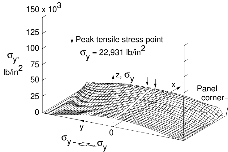
Figure 26. Distribution of \sigma_y in the lower face sheet; 4S free-edge condition; flat temperature profile; T_u = 900 °F, T_l = 200 °F.
