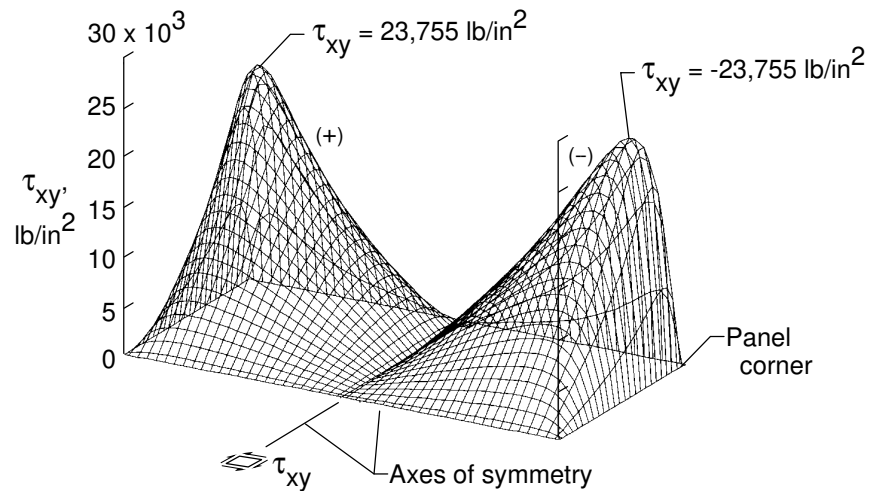
Figure 27. Distribution of \tau_{xy} in the lower face sheet; 4S free-edge condition; flat temperature profile; T_u = 900 °F, T_l = 200 °F.
