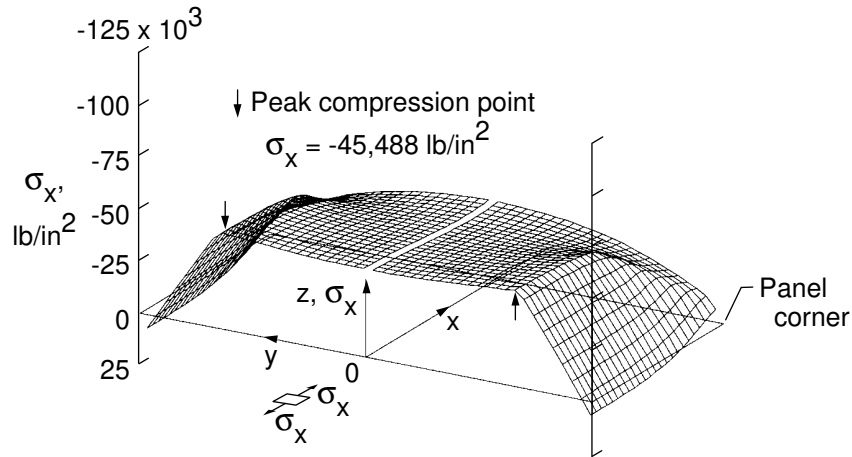
Figure 47. Distribution of \sigma_x in the upper face sheet; 4C free-edge condition; dome temperature profile; T_u = 900\text{ }^\circ\text{F} , T_l = 200\text{ }^\circ\text{F} .
