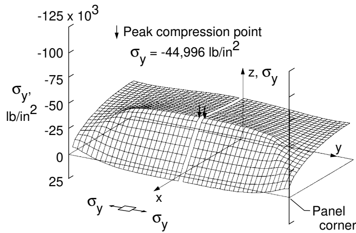
Figure 48. Distribution of \sigma_y in the upper face sheet; 4C free-edge condition; dome temperature profile; T_u = 900\text{ }^\circ\text{F} , T_l = 200\text{ }^\circ\text{F} .
