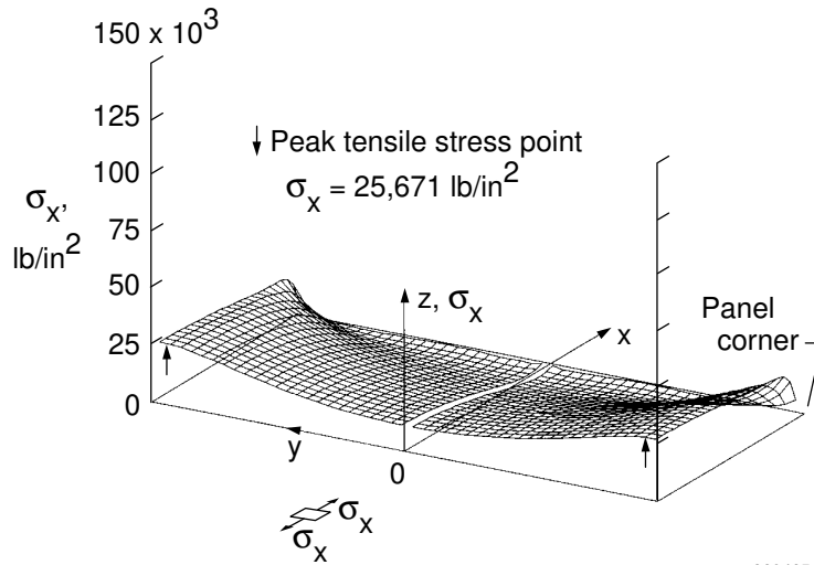
Figure 25. Distribution of \sigma_x in the lower face sheet; 4S free-edge condition; flat temperature profile; T_u = 900 °F, T_l = 200 °F.
