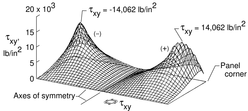
Figure 49. Distribution of \tau_{xy} in the upper face sheet; 4C free-edge condition; dome temperature profile; T_u = 900\text{ }^\circ\text{F} , T_l = 200\text{ }^\circ\text{F} .
