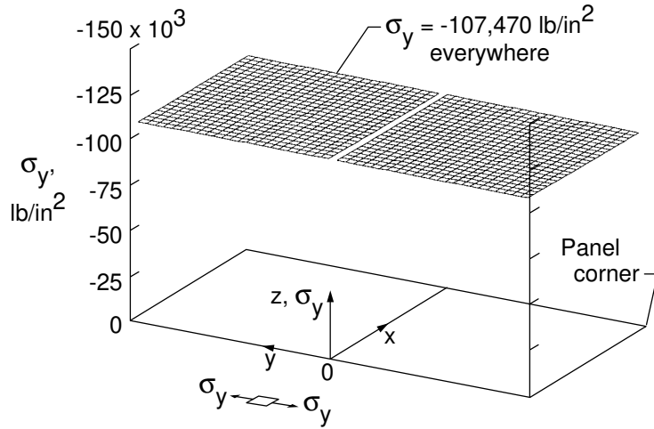
Figure 17. Distribution of \sigma_y in the upper face sheet; 4C fixed-edge condition; flat temperature profile; T_u = 900\text{ }^\circ\text{F} , T_l = 200\text{ }^\circ\text{F} .
