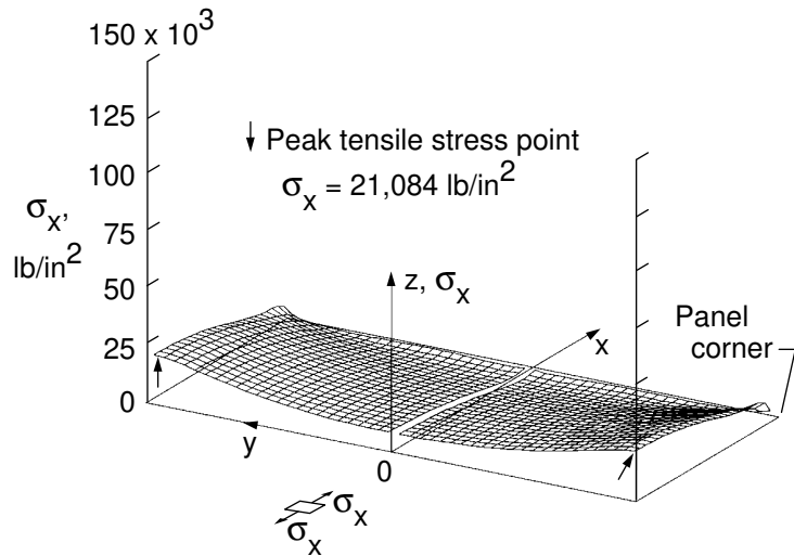
Figure 53. Distribution of \sigma_x in the lower face sheet; 4S free-edge condition; dome temperature profile; T_u = 900\text{ }^\circ\text{F} , T_l = 200\text{ }^\circ\text{F} .
