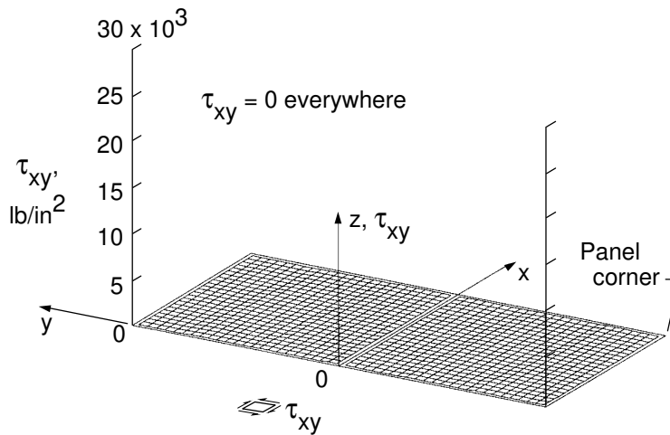
Figure 18. Distribution of \tau_{xy} in the upper face sheet; 4C fixed-edge condition; flat temperature profile; T_u = 900\text{ }^\circ\text{F} , T_l = 200\text{ }^\circ\text{F} .
