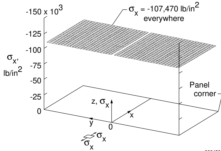
Figure 16. Distribution of \sigma_x in the upper face sheet; 4C fixed-edge condition; flat temperature profile; T_u = 900\text{ }^\circ\text{F} , T_l = 200\text{ }^\circ\text{F} .
