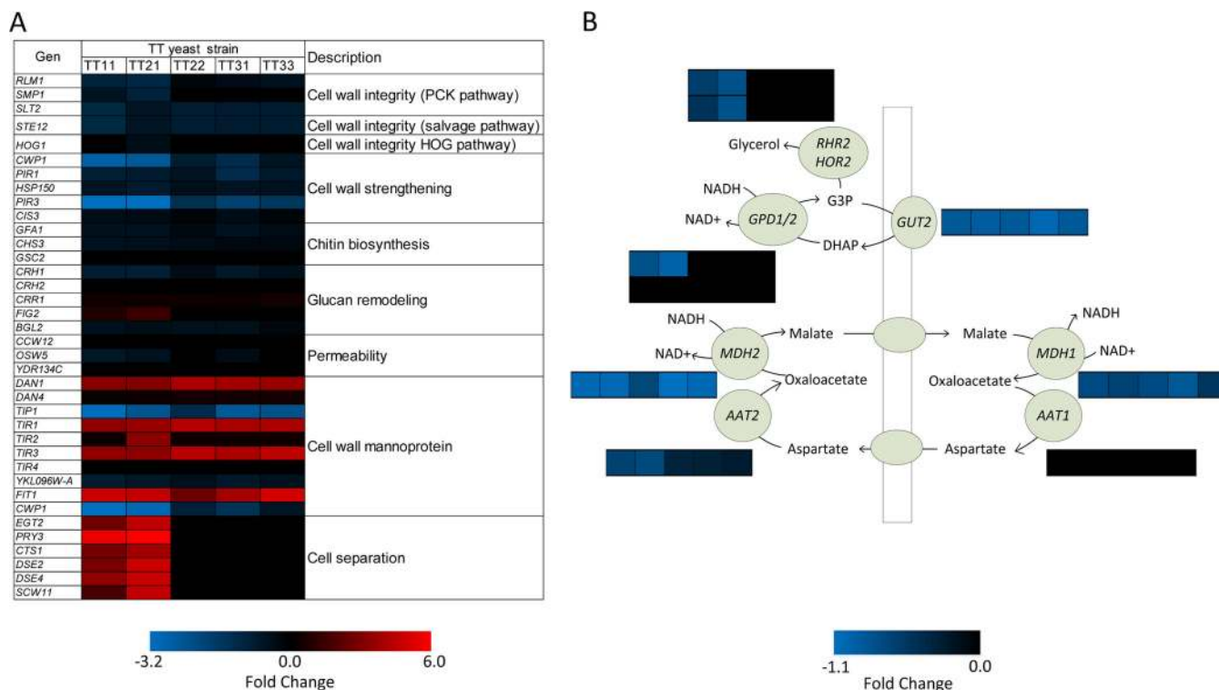
FIG 3 Transcriptional responses of thermotolerant and wild-type yeast strains growing at 40°C. (A) Changes in transcription of genes associated with stress responses related to cell wall integrity. (B) Changes in gene expression associated with glycerol synthesis and metabolism.
