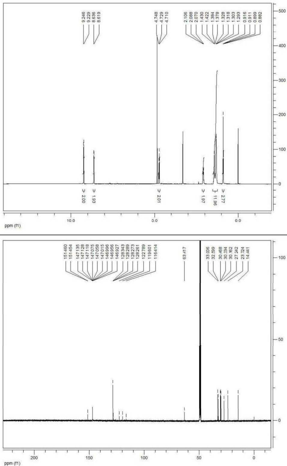
Figure S3. 1 H and 13 C NMR spectra of V9 in CD 3 OD recorded at room temperature.
