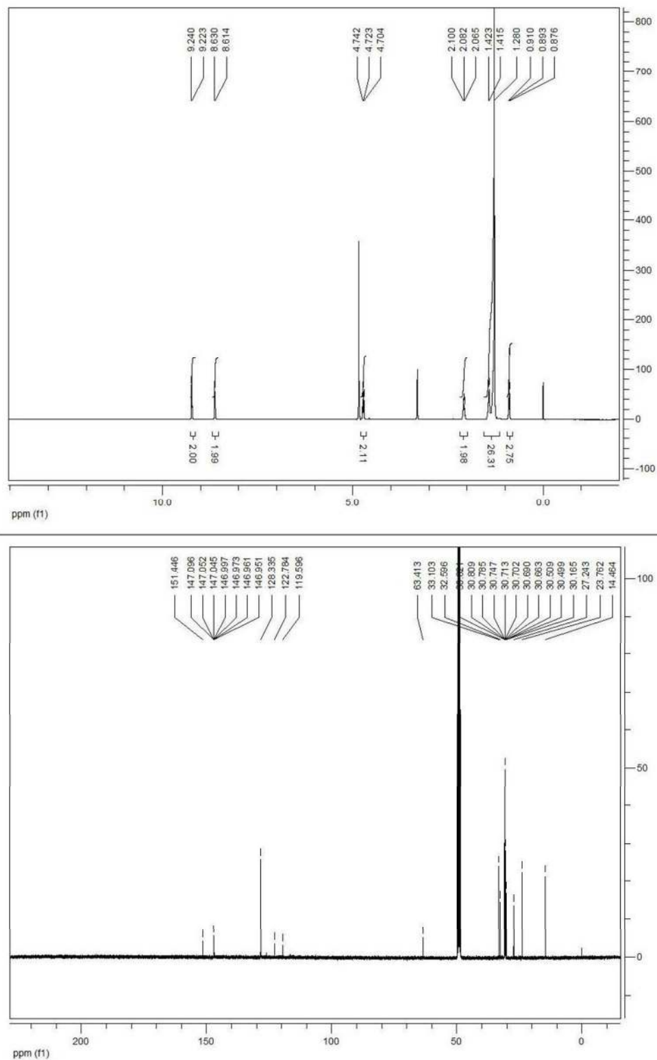
Figure S6. 1 H and 13 C NMR spectra of V16 in CD 3 OD recorded at room temperature.
