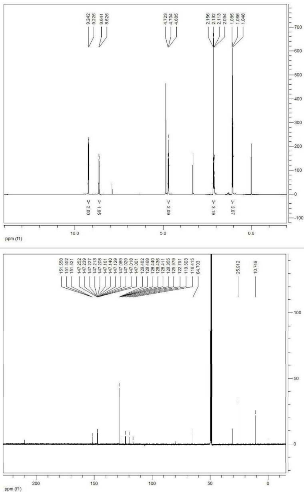
Figure S2. 1 H and 13 C NMR spectra of V3 in CD 3 OD recorded at room temperature.
