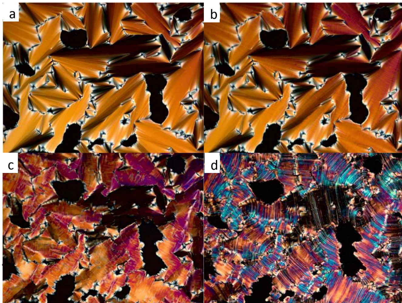
45 Figure 7. The optical textures observed in V18 when cooled from above the clearing point at 5 46 °C/min. a) The focal conic texture of V18 at 184 °C. b) The focal conic texture begins to break 47 up at 171 °C showing lines across the focal conic domains, indicating a transition to the SmC 48 phase. c) The texture of the unknown SmX phase at 113 °C. d) The texture of the crystalline 49 phase of V18 . 50
