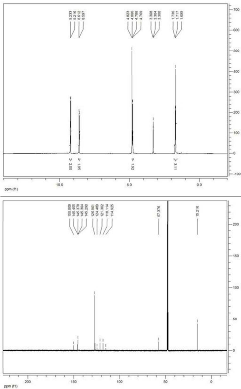
Figure S1. 1 H and 13 C NMR spectra of V2 in CD 3 OD recorded at room temperature.
