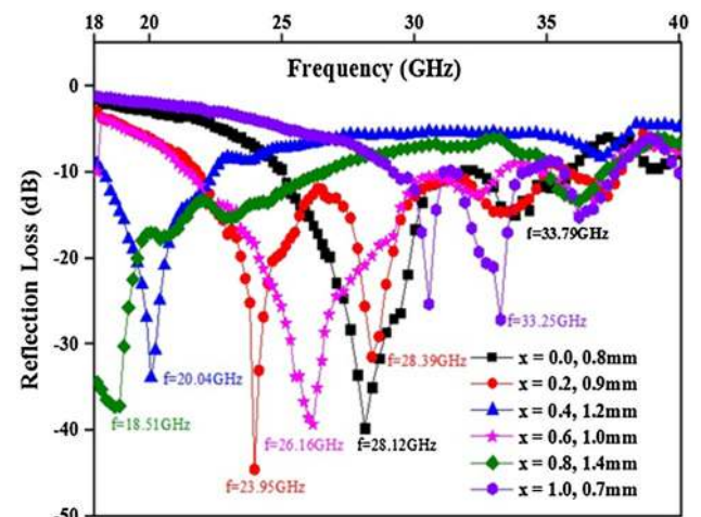
Fig. 9. Variation of RL with frequency at thickness corresponding to minimum RL value for each sample.
