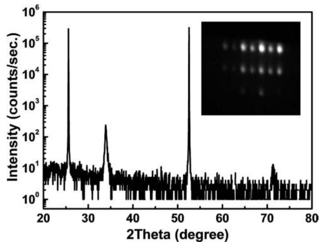
Figure 1. A typical XRD pattern of SnO 2 :Sb film on (10 \bar{1}2 ) sapphire substrate. The inset shows the in-situ RHEED pattern of the as-deposited film.
