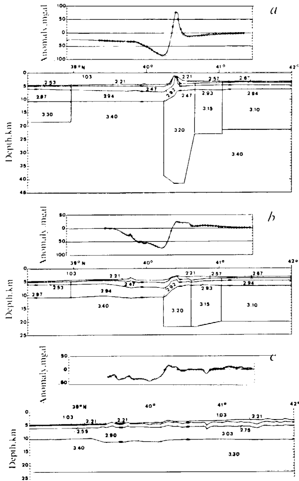
Fig. 2 Gravity profiles (free-air anomalies), and crustal sections along profiles a (along 127° 20' W), b (along 128° 20' W) and c (along 132° 30' W). In crustal sections, depth is shown from sea level, and densities ( \text{g cm}^{-3} ) are given. Data from refs 9 and 10.
