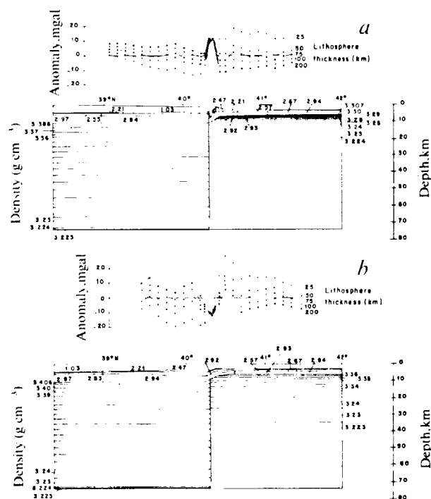
Fig. 3 Proposed density models across Mendocino Fracture Zone along profiles a and b . The thickness of the lithosphere chosen for the models is 75 km. The anomaly curves show the difference between observed and computed gravity anomalies for different lithosphere thicknesses. The density layers have been extended to infinity at both ends to avoid artificial edge effects.
