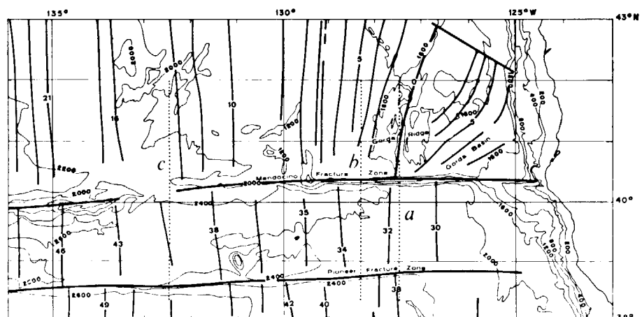
Fig. 1 Bathymetric map, after Chase et al. 18 , showing gravity profiles a , b , and c (see text). Heavy lines, magnetic lineations with ages given in Myr (after Atwater and Menard 11 ). The Mendocino Fracture Zone juxtaposes sections of lithosphere which are of different ages: across profile a , 0.3 and 31 Myr; b , 3 and 33 Myr; c , 11 and 40 Myr.
