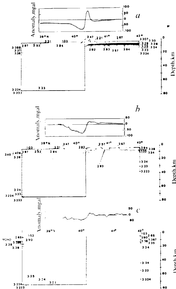
Fig. 4 Proposed density models across Mendocino Fracture Zone along profiles a , b and c and the corresponding observed (solid lines) and computed (dotted lines) gravity anomalies. The thicknesses of the lithosphere chosen for the models is 75 km. For c , the density model of the crust is a function of the age 18 (see text).
