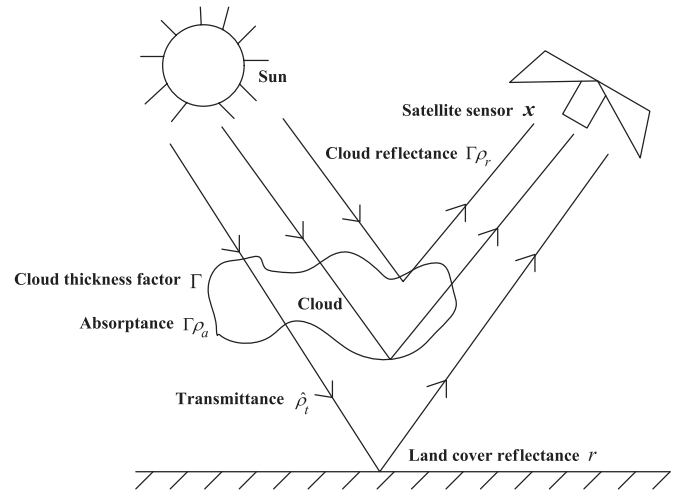
Fig. 3. Diagram of the cloud effect model.
