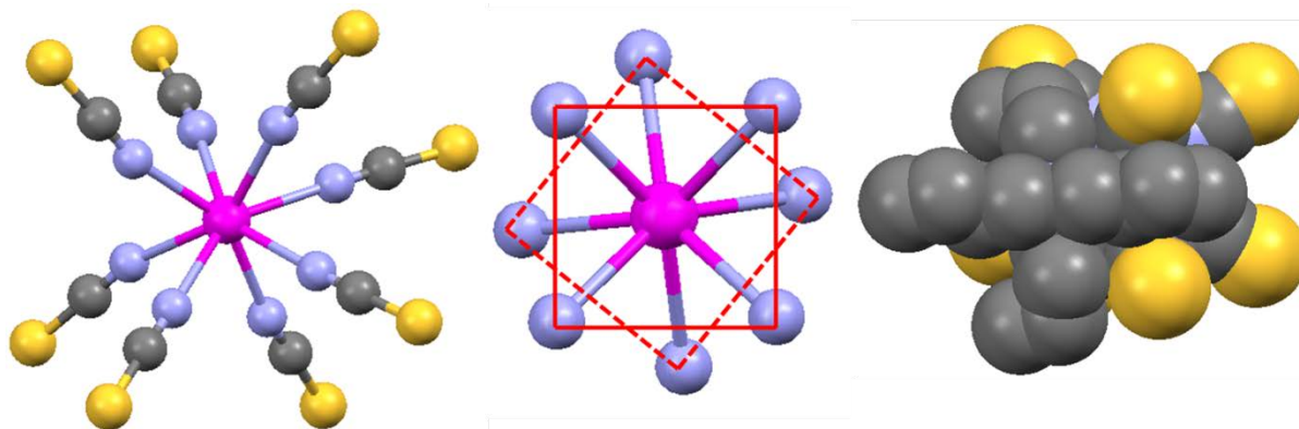
Figure 1. Solid state structure of the anion of [\text{Bu}_4\text{N}]_4[\mathbf{1}] \cdot 2\text{MeCN} (left); the coordination geometry of the uranium center (middle); the space filling diagram showing the interaction of one cation with the anion (right). Average bond lengths (Å): U–N = 2.430; N=C = 1.167; C=S = 1.628.
