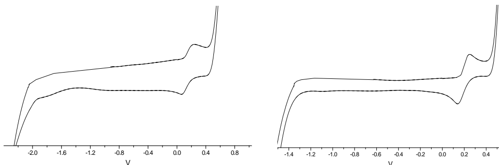
Figure 8. CV of complexes [\text{Et}_4\text{N}]_4[\mathbf{1}] (left) and [\text{Et}_4\text{N}]_4[\mathbf{2}] (right) vs \text{Fc}/\text{Fc}^+ in THF at 293 K, with \sim 0.1\text{M} [\text{Bu}_4\text{N}][\text{BPh}_4] as a supporting electrolyte (scan rate = 0.1\text{ V s}^{-1} ).
