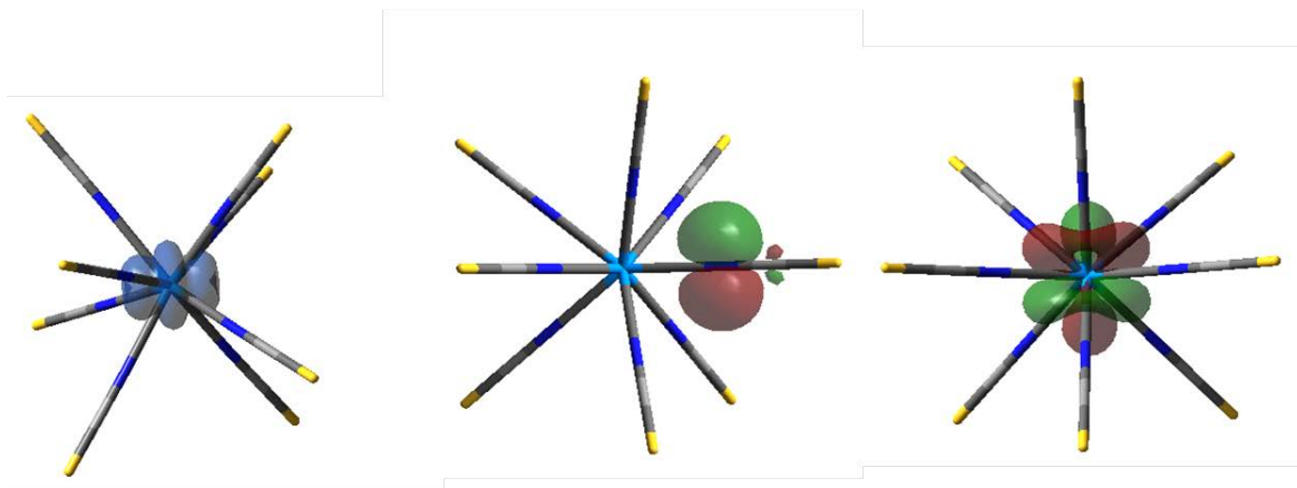
Figure 6. Spin density (left), HOMO (middle) and LUMO (right) of [1]^{4+} at the BP86 level of theory.
