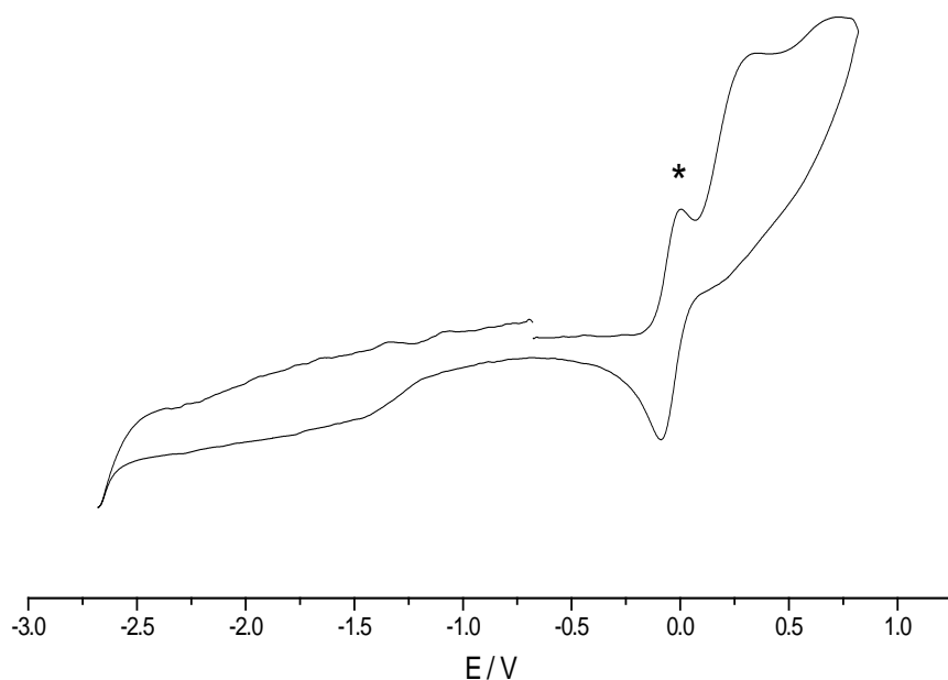
Figure 13. Cyclic voltammogram of [Et 4 N] 3 [ 3 ] in anhydrous acetonitrile/[ n Bu 4 N][PF 6 ] at 298 K.
