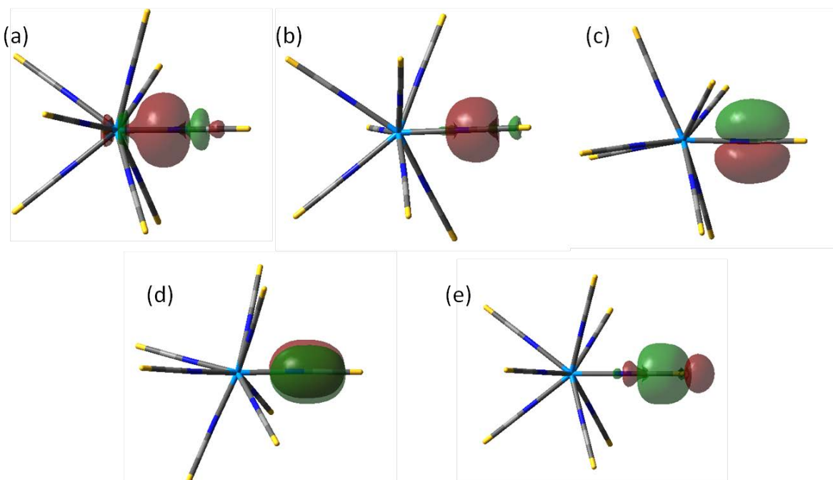
Figure 7. NBO analysis for [1]^{4+} : (a) U–N \sigma NBO; (b) N–C \sigma NBO; (c) and (d) degenerate N–C \pi NBO; (e) C–S \sigma NBO.
