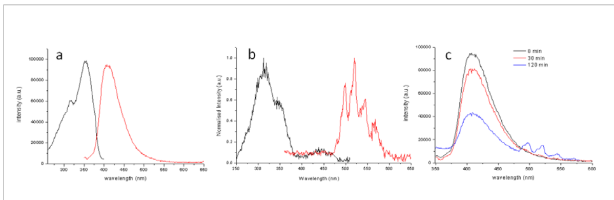
Figure 5. Excitation (black) and emission (red) spectra of (a) [Et 4 N] 4 [ 1 ] ( \lambda_{\text{ex}} = 340 \text{ nm} ; \lambda_{\text{em}} = 420 \text{ nm} ); (b) [Et 4 N] 3 [UO 2 (NCS) 5 ] ( \lambda_{\text{ex}} = 340 \text{ nm} and \lambda_{\text{em}} = 520 \text{ nm} ); and (c) emission spectra of [Et 4 N] 4 [ 1 ] exposed to air ( \lambda_{\text{ex}} = 340 \text{ nm} ), all at 298 K in CD 3 CN.
