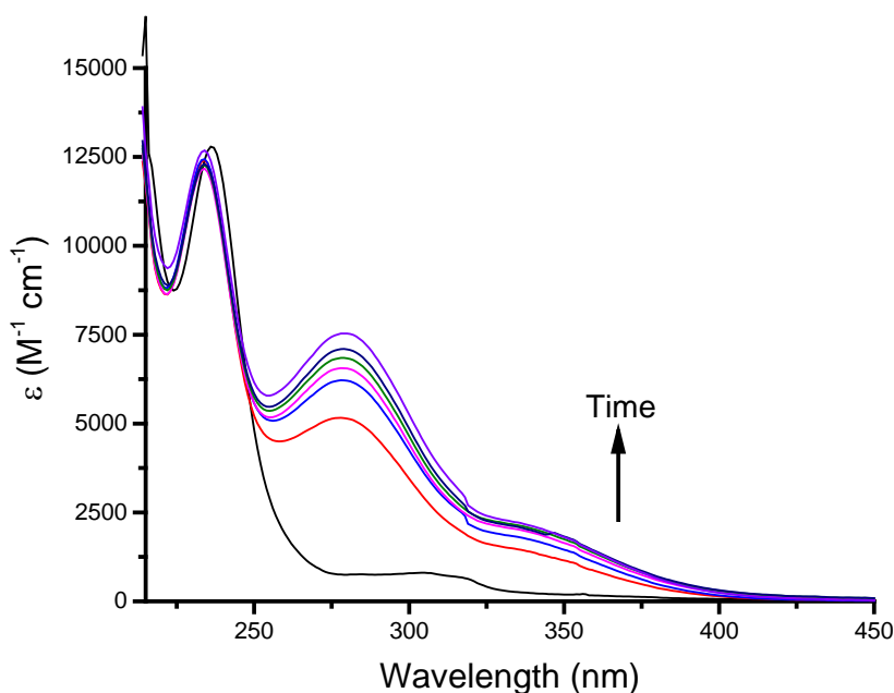
Figure 2. Changes in the UV-Vis spectrum of [Et 4 N] 4 [ 1 ] in MeCN upon exposure to UV light ( \lambda_{\text{ex}} = 340 \text{ nm} ) measured over 3 h.
