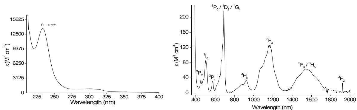
Figure 4. UV (left) and vis-NIR (right) absorption spectrum of [Et 4 N] 4 [ 1 ] in MeCN.
