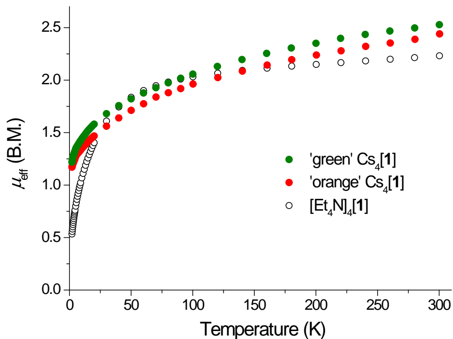
Figure 3. Magnetic susceptibility measurements, collected at 0.1 T for [Et 4 N] 4 [ 1 ] (empty bullets); ‘green’ Cs 4 [ 1 ] (green) and ‘orange’ Cs 4 [ 1 ] (red).
