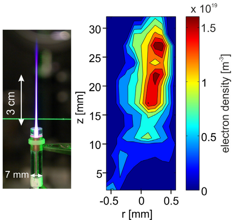
Figure 9. Pulsed DBD-like jet with a capillary inner high voltage electrode and a grounded outer ring, operated with a flow of He into ambient air, adapted from (Hübner et al 2014). For each z-position TS was recorded at the time of the maximum electron density (waveform shown in figure 10). The spatial distribution of the electron density shows its collapsing evolution. The z = 0 position corresponds to the end of the quartz tube.
