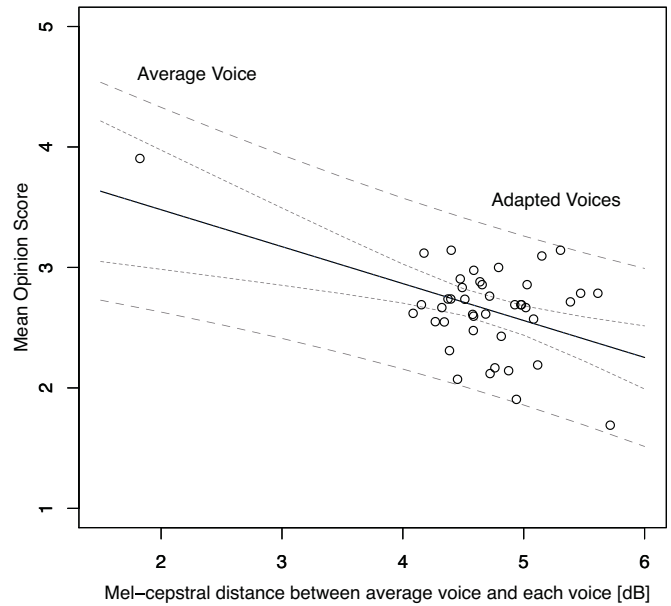
Fig. 8. The scatter plot of the mean MOS scores of 59 male voices adapted and a male average voice model. Each dot represents either the male speaker or male average voice. Horizontal axis shows the mel-cepstral distance from the average voice. Vertical axis shows the mean MOS score obtained for each voice. This also represents a linear regression function fitted and its 95% confidence and prediction intervals. For computation of the mel-cepstral distance for the average voice itself, random-sampling-based parameter generation algorithm [?] was used.
