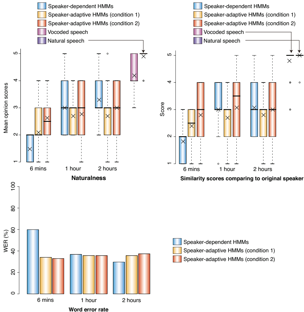
Fig. 6. Subjective evaluation results for speaker-dependent and speaker-adaptive HMM-based TTS systems built on ASR corpora. The target speaker used is a male speaker "001" included in very long subset of the WSJ0 corpus.
