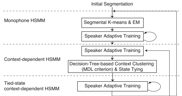
Fig. 3. Overview of the training stages for average voice models.
