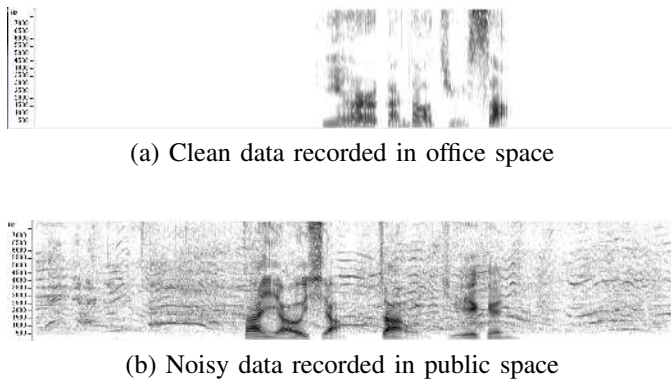
Fig. 1. Spectrograms of clean and noisy data included in the Mandarin SPEECON database.
