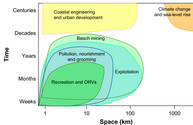
Fig. 1. Conceptual model and schematic diagram showing the relative spatio-temporal scales in which different impacts reviewed here generally operate on sandy beach macrofaunal communities. Boxes/envelopes indicate the potential extent of individual impacts in space and time with the lower curve reflecting the lower limit of impacts in time and space, whereas the upper curve reflects the corresponding maximum. Shorter term impacts (i.e., weeks to months) tend to be pulse disturbances and effects are generally expected to last for shorter time periods, since sandy-beach species are adapted to severe physical disturbances (e.g., storms). However, the temporal extent of impacts from the anthropogenic pressures depicted here could be drastically altered if the intensity of the disturbance is increased and/or its timing is more protracted. Under such circumstances, sandy beach habitats could become unsuitable for supporting macrofaunal communities and the ecosystem services they provide in the medium or long term.
