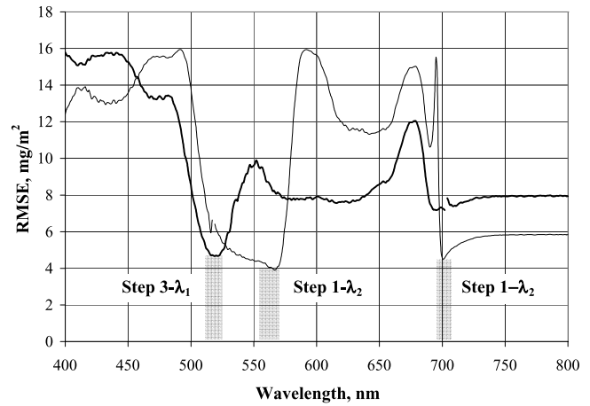
Figure 3. The first ( \lambda_2 ) and third ( \lambda_1 ) steps of model tuning for carotenoid content retrieval from reflectance spectra of 28 beech leaves with \text{Car}_{\text{mean}} = 50 \text{ mg/m}^2 . RMSE was calculated for linear regression of the [\text{R}(\lambda_1)^{-1} - \text{R}(\lambda_2)^{-1}] \times \text{R}(\lambda_3) model versus total carotenoid content.
