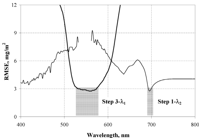
Figure 4. The first ( \lambda_2 ) and third ( \lambda_1 ) steps of model tuning for 18 dogwood leaves with \text{Anth}_{\text{mean}} = 33 \text{ mg/m}^2 . RMSE was calculated for linear regression of the [R(\lambda_1)^{-1} - R(\lambda_2)^{-1}] \times R(\lambda_3) model versus anthocyanin content.
