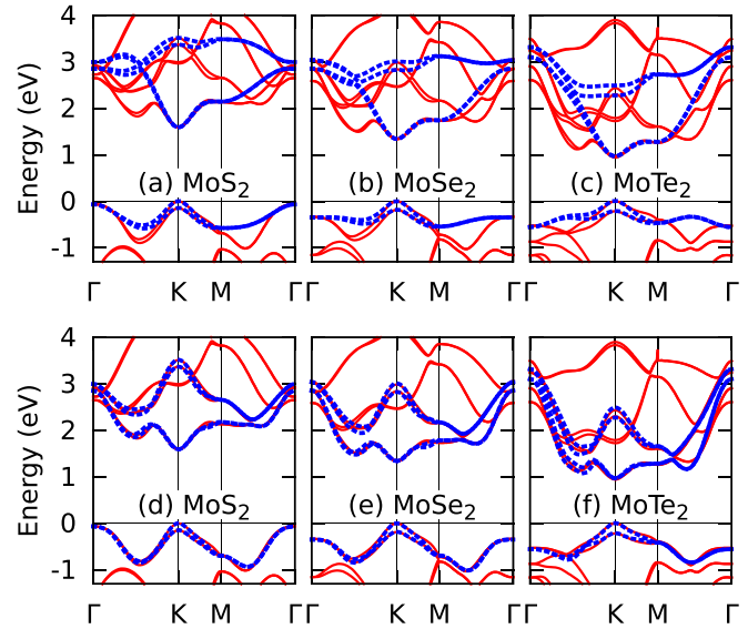
FIG. 6. (Color online) Energy bands of monolayers MoX_2 with SOC. Thick blue dashed curves are the TB bands: (a–c) from the NN TB model and (d–f) from the TNN TB model. Thin red solid curves are FP results with GGA. VBMs are shifted to zero.
