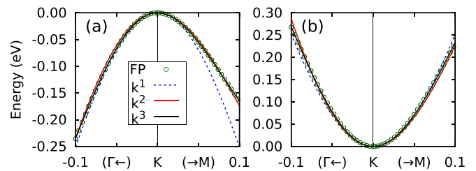
FIG. 10. (Color online) (a) Valence and (b) conduction bands in the K valley of monolayer MoS 2 , within the range of 0.1 \times \frac{2\pi}{a} in \Gamma and M directions. Open circles are FP results (GGA case). Blue dashed, red solid, and black solid curves are the bands from the two-band \mathbf{k} \cdot \mathbf{p} model of H_{kp}^{(1)} , H_{kp}^{(2)} , and H_{kp}^{(3)} , respectively. CBMs and VBMs are both shifted to 0. a = 3.190 Å and \Delta = 1.663 eV for all. Other fitted parameters are the following: t = 1.105 eV for H_{kp}^{(1)} ; t = 1.059 eV, \gamma_1 = 0.055 eV, \gamma_2 = 0.077 eV, and \gamma_3 = -0.123 eV for H_{kp}^{(2)} ; t = 1.003 eV, \gamma_1 = 0.196 eV, \gamma_2 = -0.065 eV, \gamma_3 = -0.248 eV, \gamma_4 = 0.163 eV, \gamma_5 = -0.094 eV, and \gamma_6 = -0.232 eV for H_{kp}^{(3)} .
