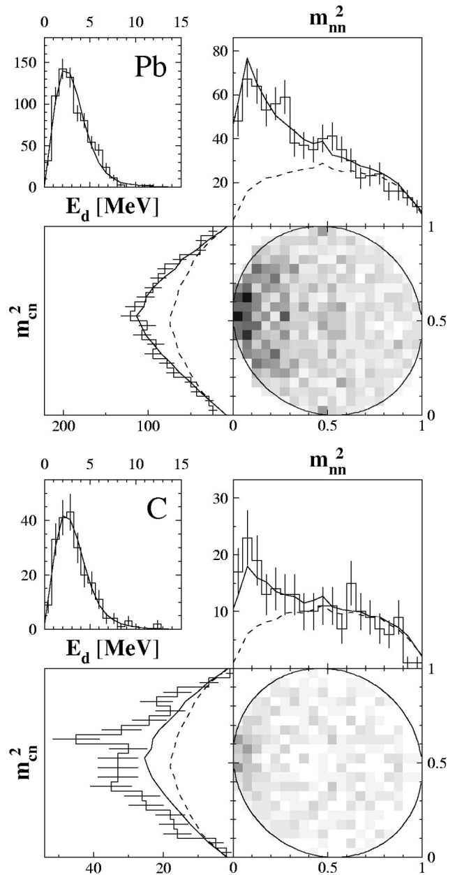
FIG. 3. Dalitz plots (core- n vs n - n ), and the projections onto both axes, for the data from the dissociation of ^{14}\text{Be} by Pb (upper panels) and C (lower panels). The lines are the results of the phase-space model simulations with/without (solid/dashed) n - n FSI. The insets correspond to the ^{14}\text{Be} decay energy.
