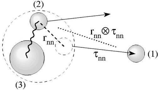
FIG. 1. Schematic view of the sequential breakup of a two-neutron halo nucleus, whereby dissociation passes through a resonance in the core- n system. A delay \tau_{nn} , equivalent to the lifetime of the resonance, is introduced in the emission of the second neutron. The effective source size is a convolution of the n - n separation r_{nn} and the delay \tau_{nn} .
