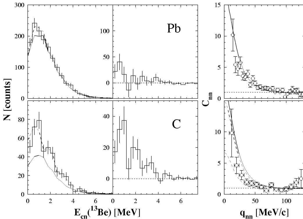
FIG. 4. Core- n relative energy distributions and n - n correlation functions for the dissociation of ^{14}\text{Be} by Pb (upper panels) and C (lower panels). The lines in the E_{cn} spectra (left) are the result of the phase-space model simulations with n - n FSI (solid lines) plus core- n resonances (dashed lines, see text). The histograms presented in the middle panels are the difference between the data and the n - n FSI simulations. The solid lines in the right panels are the C_{nn} for r_{nn}^{\text{rms}}=5.6 fm and \tau_{nn}=0 ; the dashed lines correspond to the limits r_{nn}^{\text{rms}}=6.6\text{--}4.6 fm and \tau_{nn}=0\text{--}400 fm/ c .
