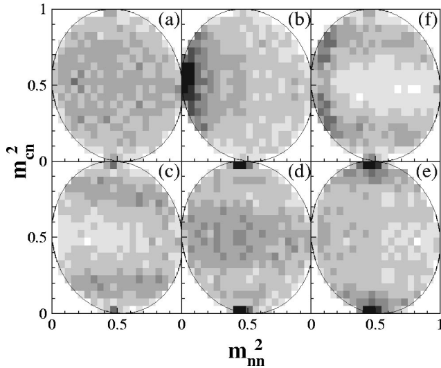
FIG. 2. Dalitz plots (core- n vs n - n ) for simulations with the interacting phase-space model of ^{14}\text{Be} dissociation: without FSI (a), with n - n FSI (b), and with a core- n resonance at E_0=0.8 (c), 2.0 (d), and 3.5 MeV (e). The combination of the n - n and the core- n FSI of (c) is shown in (f).
