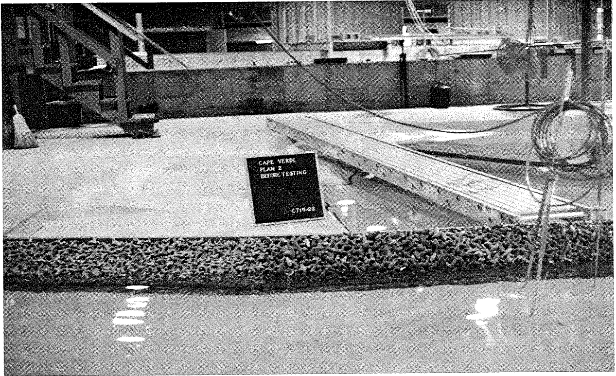
Photo A23. Sea-side view of plan 2 breakwater trunk before testing
