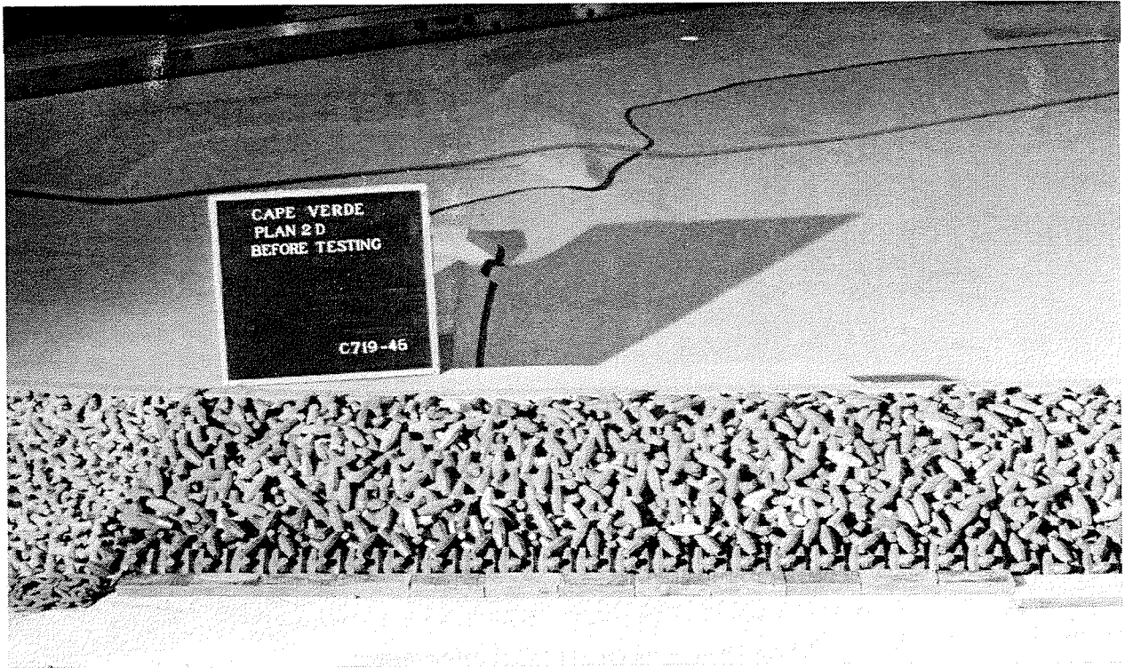
Photo A43. Sea-side view of plan 2D, profiles 4 through 6, before testing
