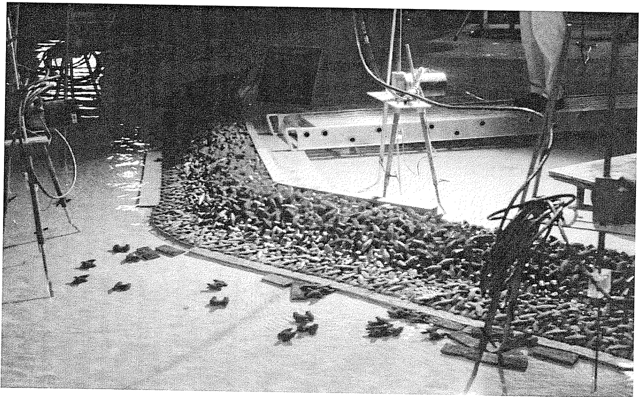
Photo A46. Sea-side view of plan 2D breakwater head after testing with total storm sequence
