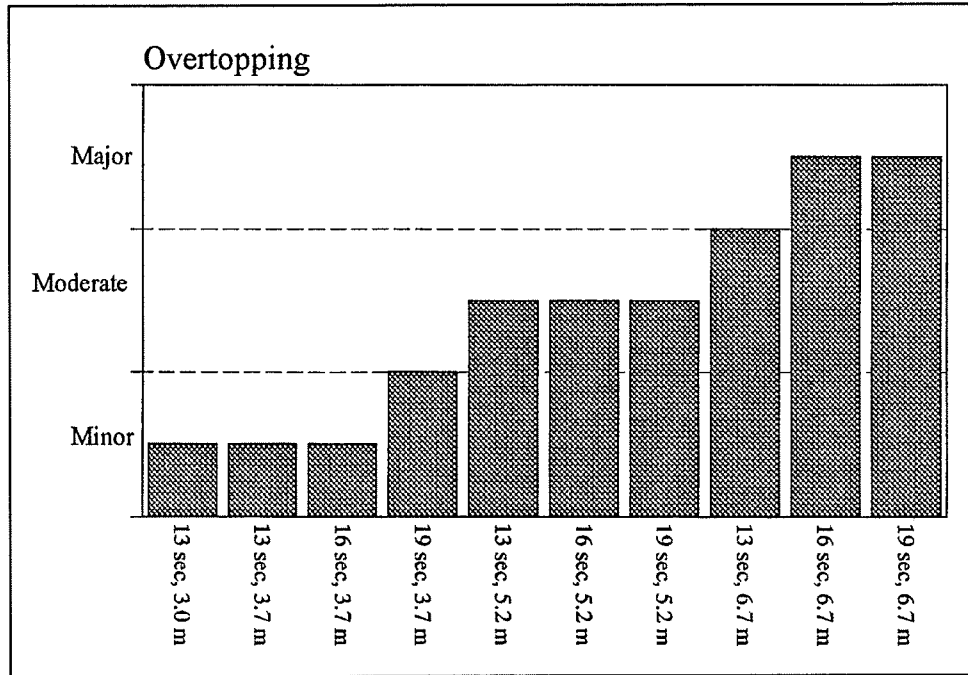
Figure 17. Wave overtopping at trunk, all plans
