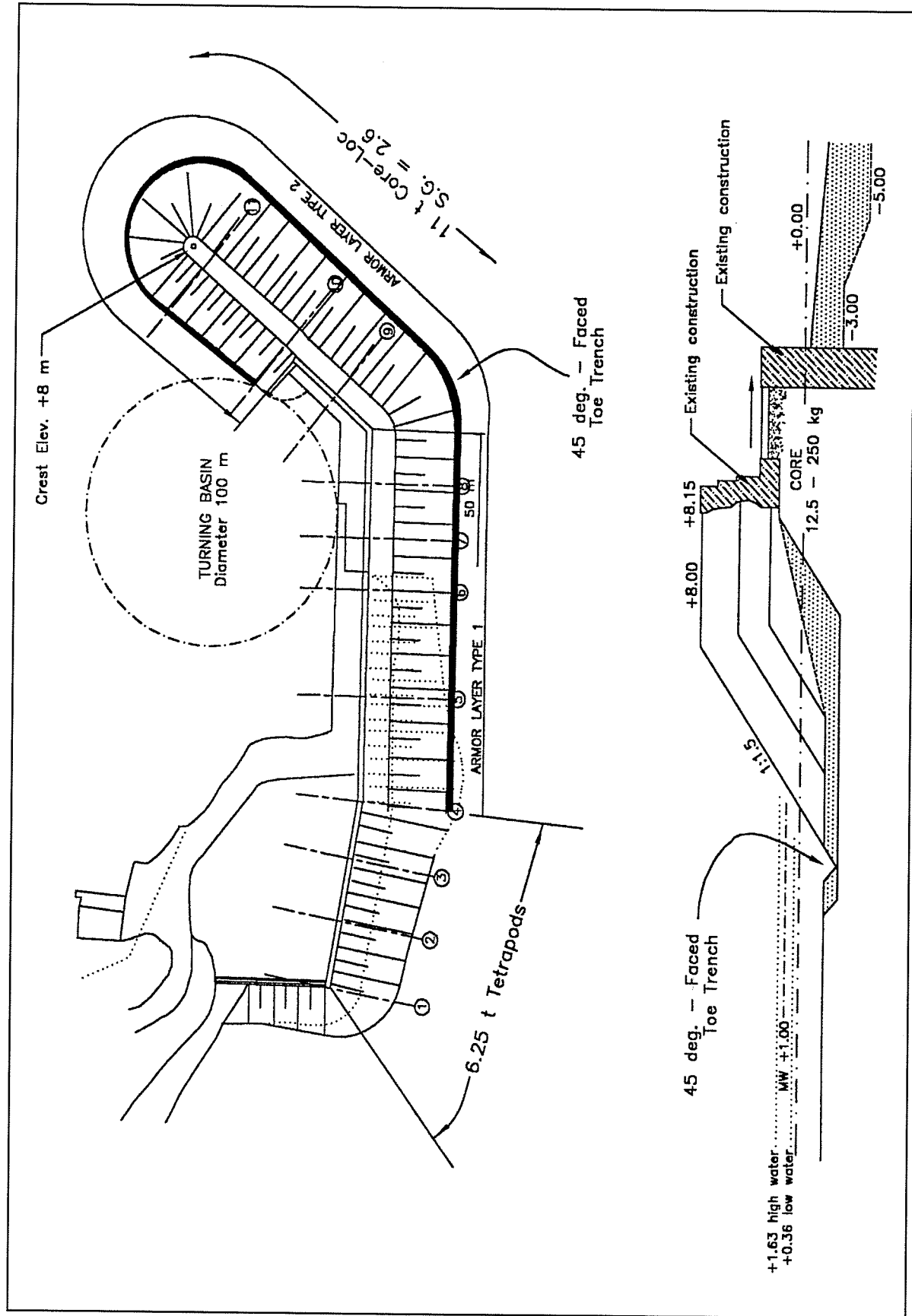
21 Figure 14. Elements of plan 2A
