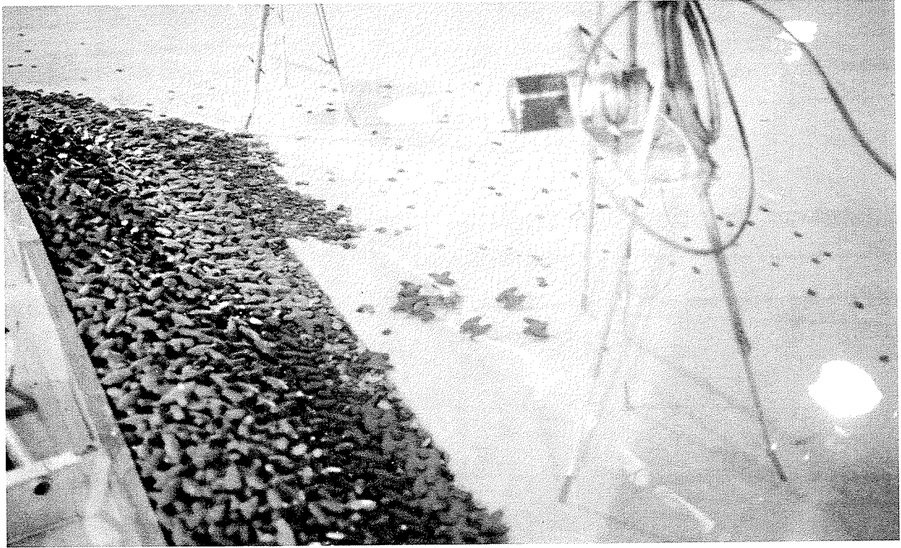
Photo A27. View of plan 2 breakwater trunk, profiles 6 to 8, after testing with 15-sec and 16-sec waves
