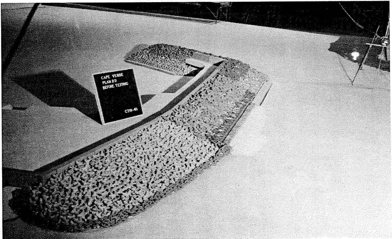
Photo A44. View from north of plan 2D breakwater trunk before testing
