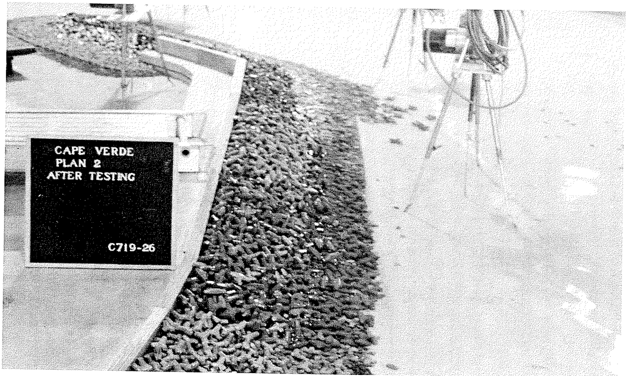
Photo A26. View from north of plan 2 breakwater trunk after testing with 13- and 16-sec, 3.7-m waves
