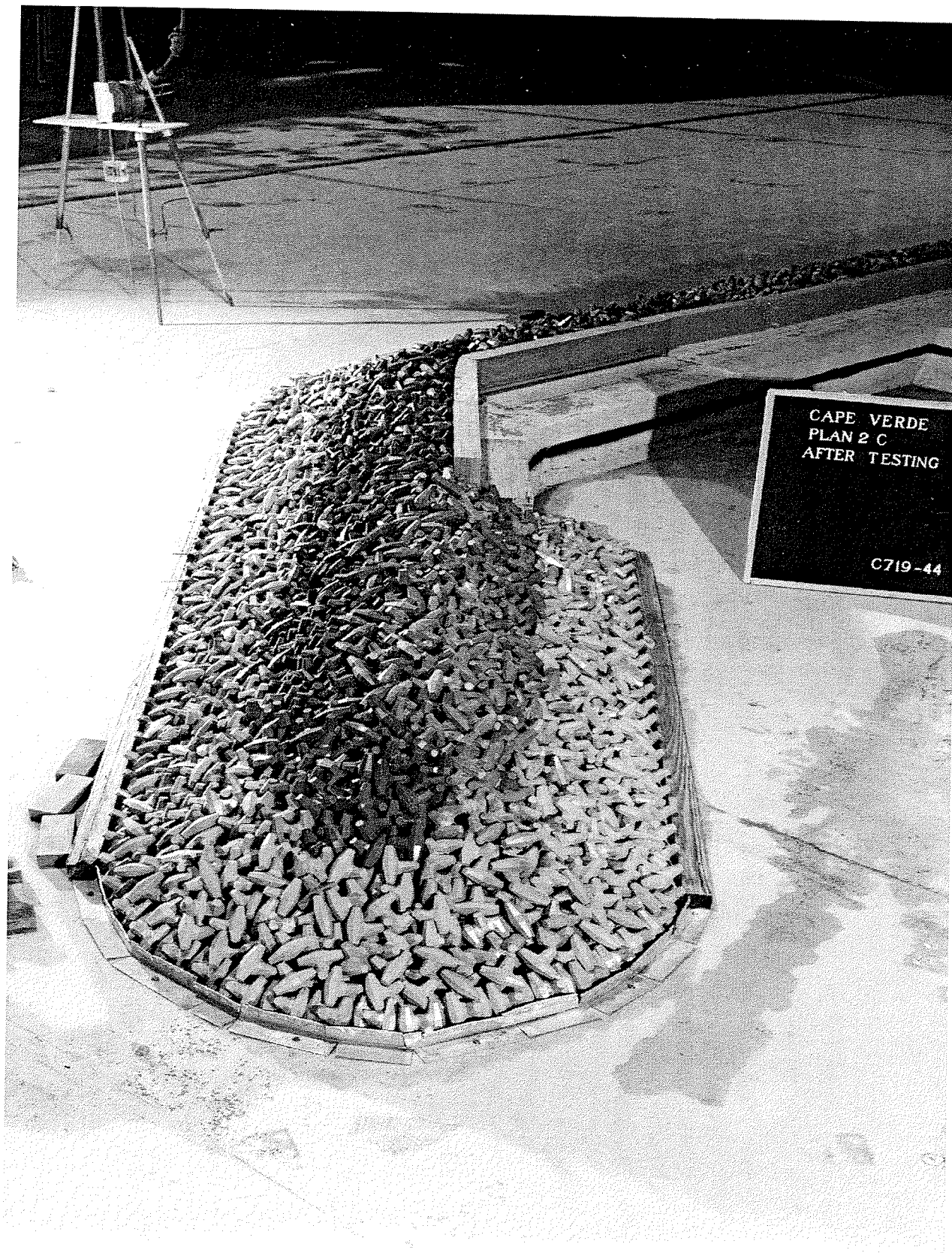
Photo A42. View of plan 2C breakwater head after testing with waves above the 3.7-m height
