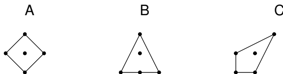
Figure 5. Three toric diagrams which have pure SU(2) gauge theory description along certain locus of Coulomb branch.
