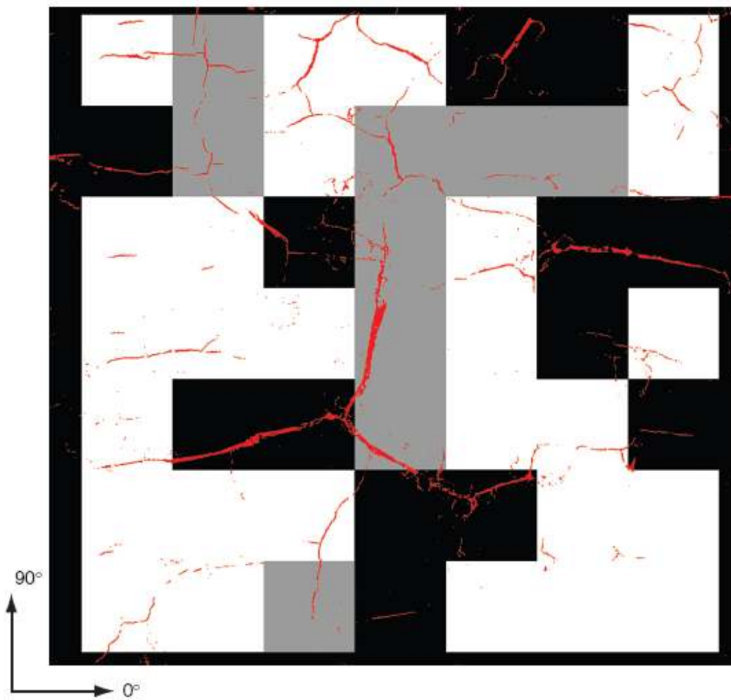
Figure 8 Mean crack orientation at the final stage : white squares represent units with l_c \inf < A A l < l_c \sup , grey squares represent units with A A > l_c \sup , and black squares represent units with A A < l_c \inf .
