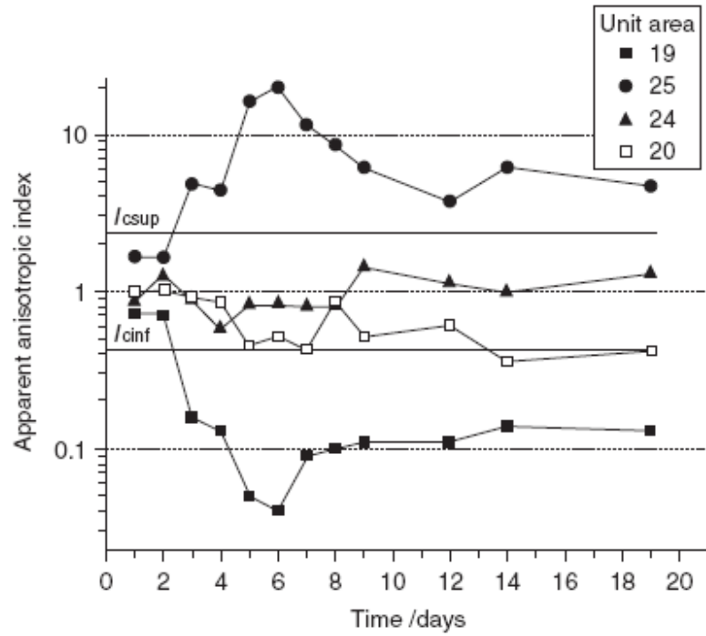
Figure 12 Variation of AAI and comparison with I_{cinf} and I_{csup} thresholds during drying for the four unit areas 19, 25, 24 and 20.
