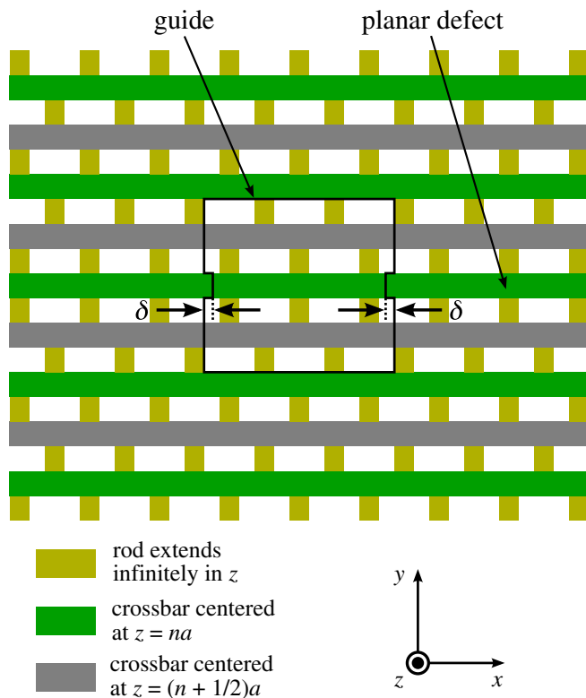
FIG. 2. The geometry of a vertically symmetric waveguide structure.
