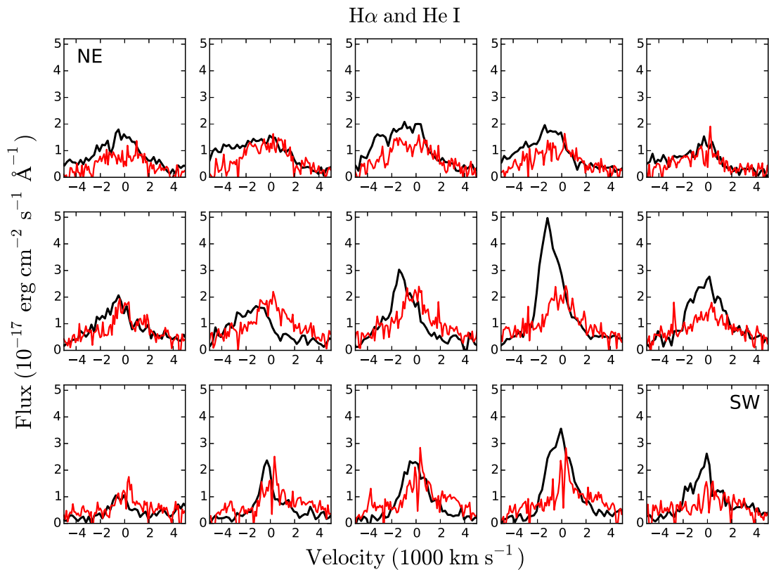
Figure 21. Comparison of the H \alpha (black) and He I 2.058 \mu\text{m} (red) lines extracted from the regions shown in Figure 8. The SINFONI spectrum of He I has been multiplied by a factor of 20.
