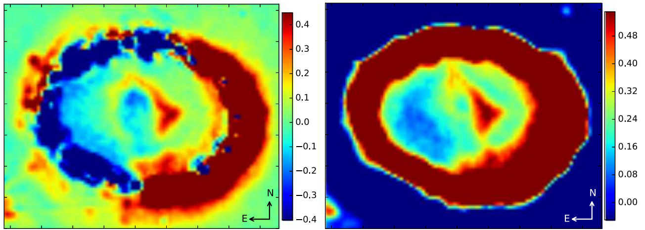
Figure 13. HST F625W difference images between days 9973 and 6790, showing the evolution of H\alpha . These images are close in time to the spectra from days 10,035 and 6355 shown in Figure 12. In the right panel the image from day 6790 was expanded by a factor of 1.5 before the subtraction in order to account for the expansion of the ejecta between the two epochs. As a result, this image does not provide any information about the evolution of the ring. The color bars show the intensity in units of 2.5 \times 10^{-16} \text{ erg cm}^{-2} \text{ s}^{-1} . A comparison between these images and Figure 12 confirms that the flux increase in the range [-2000, 0] \text{ km s}^{-1} is primarily driven by the western clump. There is also a significant increase in the southern ejecta, but about half of this region is outside the spectral extraction box (see Figure 6) due to the spatial overlap with the ring. The bright region at the inner edge of the ring in the west is due to the reverse shock.
