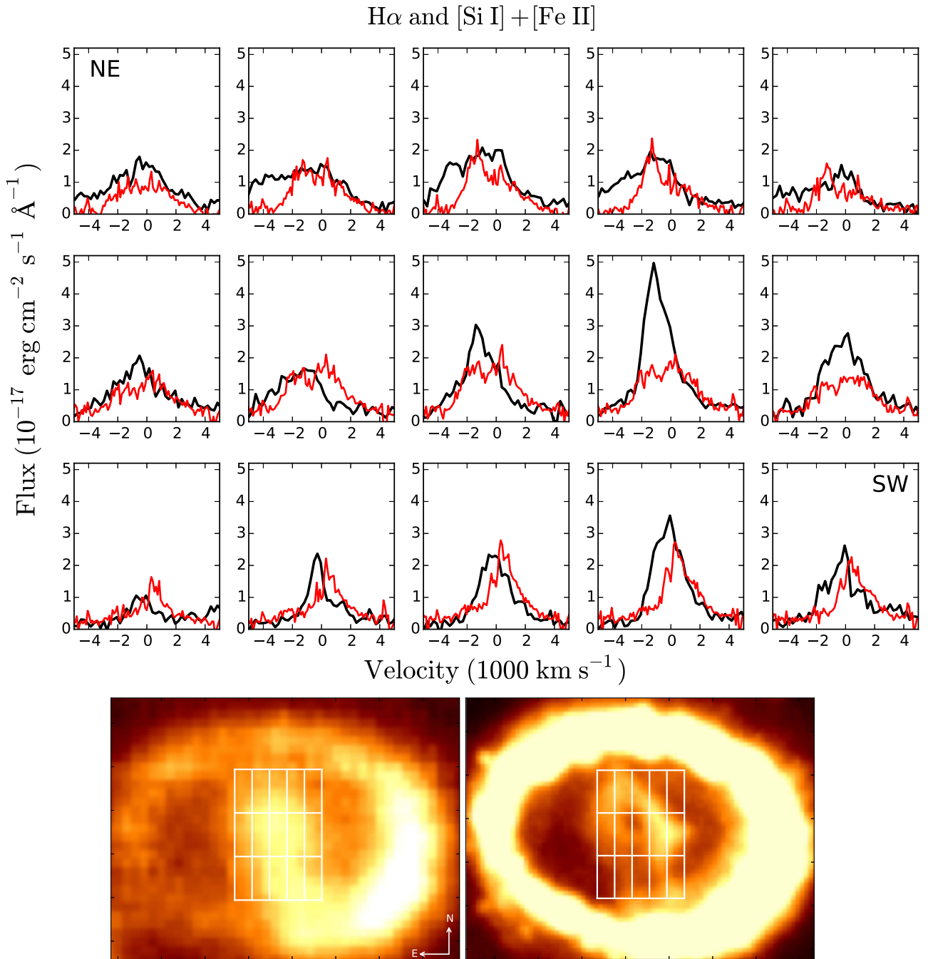
Figure 8. Comparison of the [\text{Si I}] + [\text{Fe II}] (red) lines and H\alpha (black) extracted from 0''.1 \times 0''.25 regions of the ejecta. The regions are shown in the bottom panel, superposed on the image of the 1.644 \mu\text{m} , \pm 3000 \text{ km s}^{-1} line (left) and the WFC3/F625W image (right). The panels with the line profiles are organized in the same way as the regions, with the upper left panel corresponding to the region in the northeast corner. The spectra have been corrected for emission from the ring as demonstrated in Figures 6 and 7. The SINFONI spectra have been multiplied by a factor of 10 to match the flux level of the STIS spectra.
