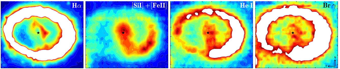
Figure 5. Contour plots of the ejecta in different lines. The left panel was produced from the WFC3 F625W image in Figure 1, which is dominated by emission from H\alpha . The next three panels show emission from [\text{Si I}] + [\text{Fe II}] , \text{He I} , and \text{Br}\gamma , respectively. These three panels were produced from SINFONI data, covering \pm 3000 \text{ km s}^{-1} around each line with the central \pm 450 \text{ km s}^{-1} removed. The latter cut removes most of the contribution from the narrow lines from the ring. The remaining emission from the ring seen in the images is primarily continuum emission. This is particularly strong in the southwest part of the ring. The contours in each plot are linearly spaced in flux between the maximum (red) and minimum (blue) of the ejecta region. The ring is shown in white in those parts where it is brighter than the maximum of the ejecta region. The black star marks the geometric center of the ring.
