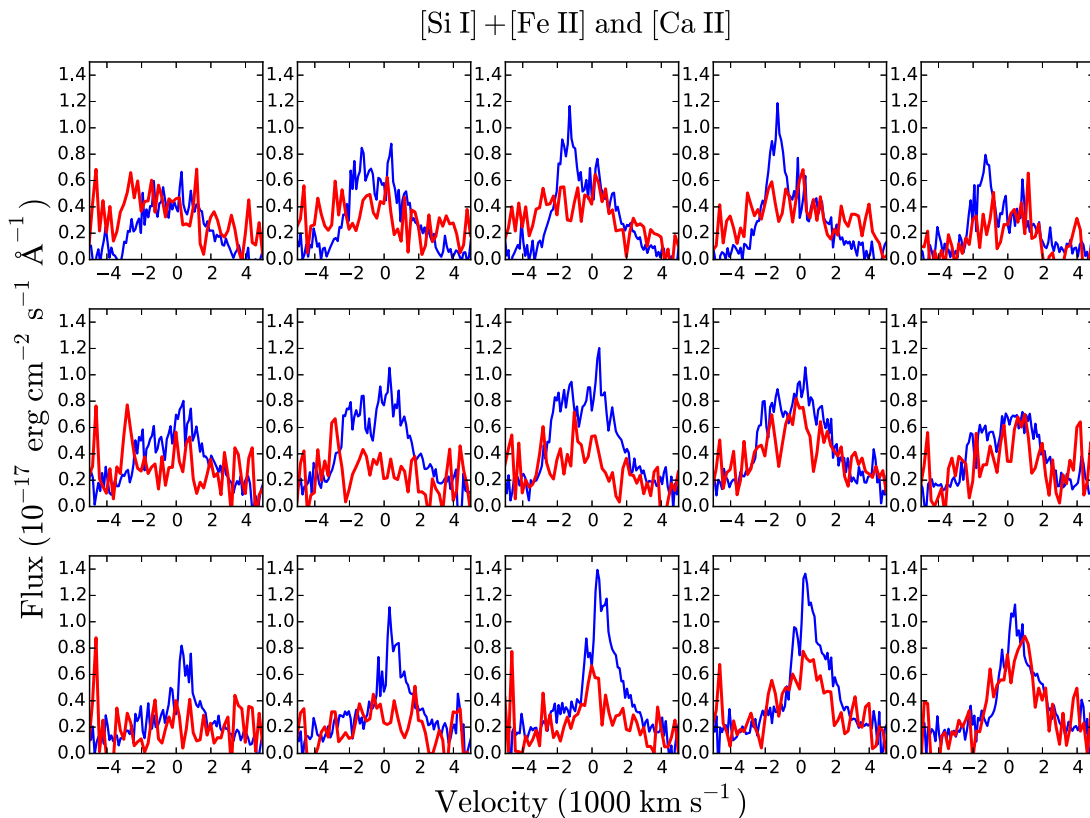
Figure 19. Comparison of the [Si I] + [Fe II] 1.644 \mu\text{m} (blue) and [Ca II] \lambda\lambda 7292, 7324 (red) lines extracted from the regions shown in Figure 8. The spectrum has been multiplied by a factor of five for [Si I] + [Fe II] . For [Ca II] the spectrum is centered on zero velocity for the average wavelength of the two components.
