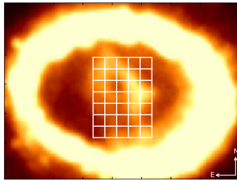
Figure 6. Spatially resolved STIS G750L spectra of H\alpha , extracted from 0''.1 \times 0''.1 regions of the ejecta. The regions are shown superposed on the WFC3/F625W image in the bottom panel. The panels with the line profiles are organized in the same way as the regions, with the upper left panel corresponding to the region in the northeast corner. At this epoch 0''.1 corresponds to 866 \text{ km s}^{-1} . The dashed and solid lines show the spectra before and after correcting for scattered light from the ring, respectively.
