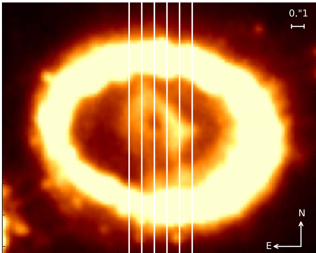
Figure 1. Slit positions for the STIS observations from day 10,035 shown superposed on the WFC3/F625W image from day 9973. The slit width is 0''.1 . The ring has a radius of approximately 0''.8 ( \sim 0.6 lt-yr) and an inclination of 44^\circ (Plait et al. 1995).
