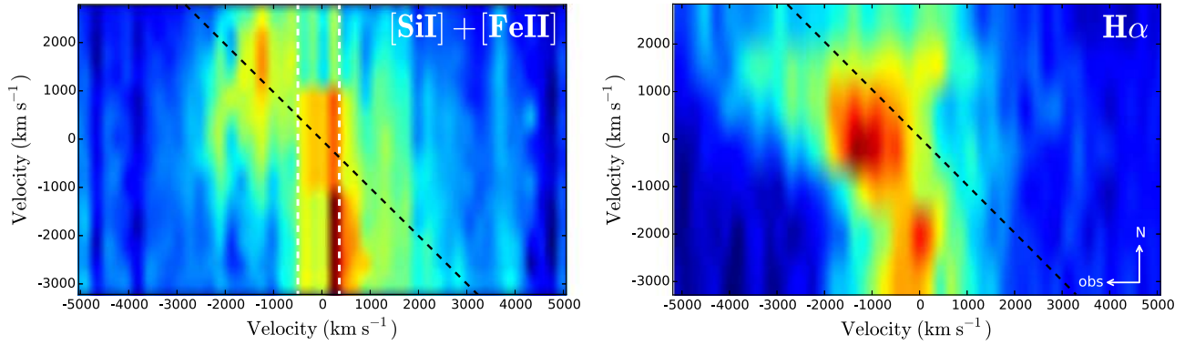
Figure 10. Side views of the ejecta for [Si I]+[Fe II] (left) and H\alpha (right). The observer is located to the left and the plane of the ring is indicated by the dashed, black line. The spatial region covered is the same as in Figure 9. The spatial scale was converted to a velocity scale in the north–south direction using the relation 0^\circ 1 = 866 \text{km s}^{-1} . The SINFONI spectra have been binned by a factor of six compared with the original resolution. Both data sets have been corrected for emission from the ring and smoothed by a 2D spline function. In the case of [Si I]+[Fe II], the ring correction results in a significantly lower resolution (by a factor of five) in the north–south direction inside the region marked by the white dashed lines. The color scale is set between the maximum (red) and minimum (blue) of each image.
