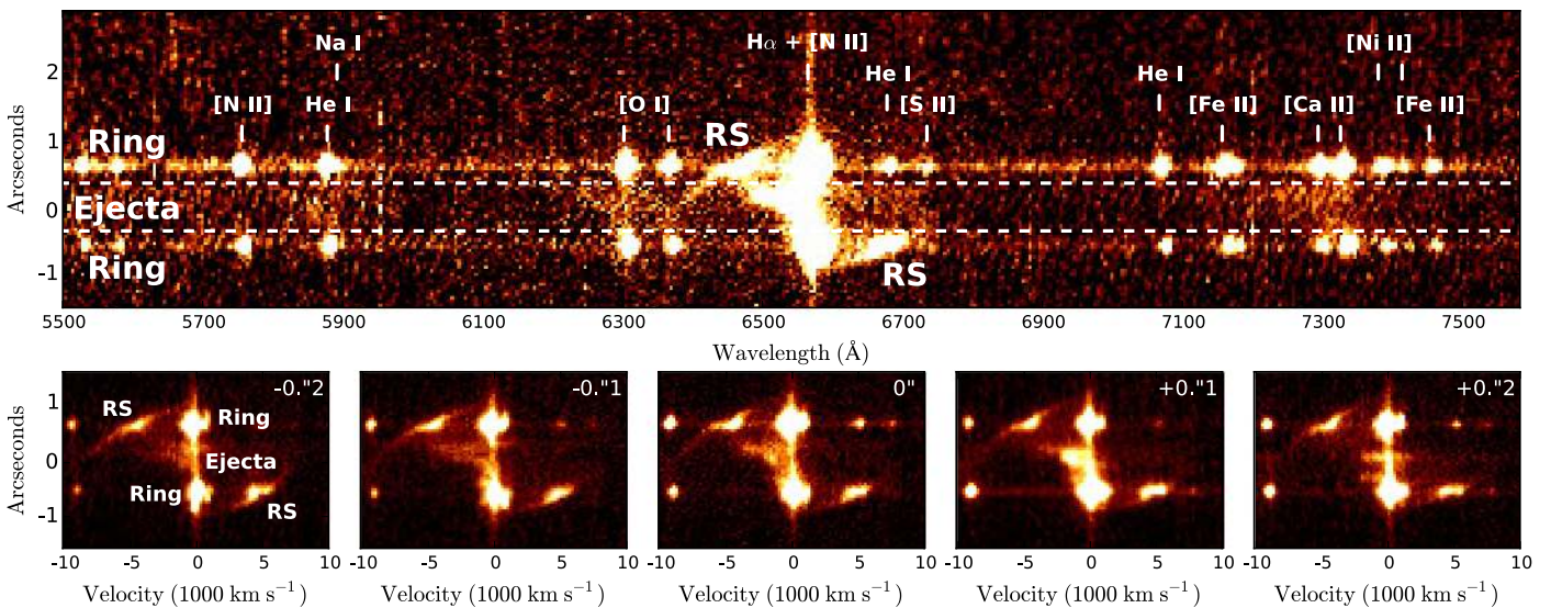
Figure 2. Two-dimensional STIS G750L spectra. Upper panel: spectrum from the central slit position in Figure 1 with all emission lines identified. The main emission components are also labeled: the ring, the ejecta, and the reverse shock (RS). The latter is seen only in H \alpha . The dashed lines show the region used to extract the ejecta spectrum in Figure 3. Significant emission from the ejecta is detected in Na I \lambda\lambda 5890, 5896 , [O I] \lambda\lambda 6300, 6364 , H \alpha , [Ca II] \lambda\lambda 7292, 7324 , as well as Mg II \lambda\lambda 9218, 9244 . The latter lines are outside the plotted region but shown in Figure 3. Bottom panels: emission from H \alpha for all five slit positions in Figure 1, with the leftmost panel corresponding to the position furthest to the east, etc. The main emission components are also indicated in the left panel.
