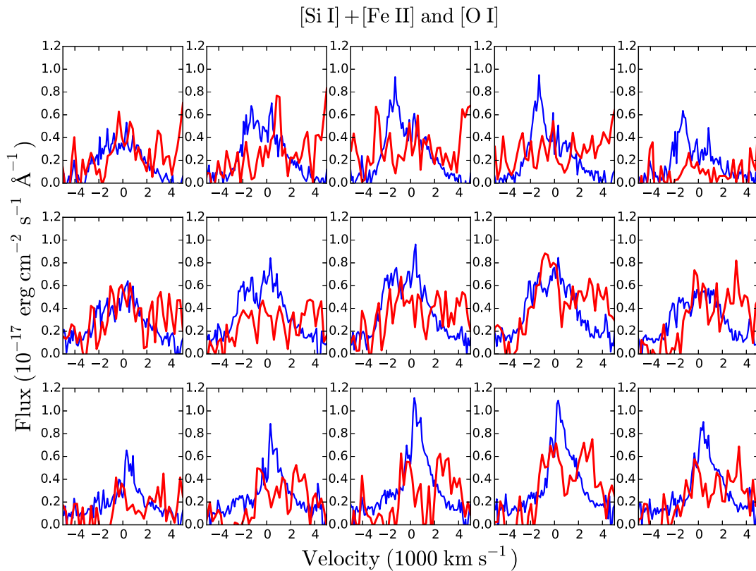
Figure 17. Comparison of the [Si I]+[Fe II] 1.644 \mu\text{m} (blue) and [O I] \lambda\lambda 6300, 6364 (red) lines extracted from the regions shown in Figure 8. The spectrum has been multiplied by a factor of four for [Si I]+[Fe II]. For [O I] the spectrum is centered on zero velocity for the 6300 Å component.
