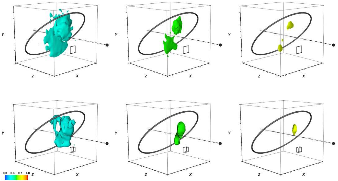
Figure 11. 3D iso-surfaces for [Si I]+[Fe II] (top row) and H\alpha (bottom row). Plots from left to right show the contours corresponding to 30%, 50%, and 70% of the maximal intensity of each line, as indicated by the color bar. The ring shows the location of the reverse shock at the inner edge of the equatorial ring, while the dotted line and filled sphere indicate the line of sight and the position of the observer. The tick marks on the axes correspond to 1000 \text{ km s}^{-1} . The boxes to the lower right of each plot show the resolution along the three axes. The [Si I]+[Fe II] plots include all data out to 4500 \text{ km s}^{-1} in all directions, with the central \pm 450 \text{ km s}^{-1} along the line of sight removed due to contamination from the ring. The latter cut creates a gap in the center, although it is not seen in the top left panel due to projection effects. The data cube was binned by a factor of six in the spectral direction. The H\alpha plots were created from the ring-corrected spectra in Figure 6, which cover [-2000, +2300] \text{ km s}^{-1} in the x -direction and [-3300, +2800] \text{ km s}^{-1} in the y -direction. The main effect of these cuts is that some of the bright ejecta in the south is excluded (see the lower right panel of Figure 9). Along the line of sight, all data within \pm 4500 \text{ km s}^{-1} are included. Animated versions of this figure are available in the online journal. The first animation shows the top row from different viewing angles, while the second one is a semi-transparent version showing multiple contour levels simultaneously. The third and fourth animations are the same, but for the bottom row.
