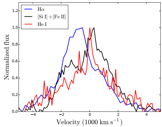
Figure 4. Comparison of the velocity profiles of the three strongest lines from the ejecta: H\alpha , [Si I]+[Fe II] 1.644 \mu\text{m} , and He I 2.058 \mu\text{m} . The lines have been normalized to the same maximum value after subtracting the continuum. The SINFONI spectra have been binned by a factor of three.
