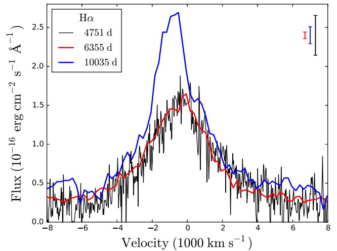
Figure 12. Time evolution of the H \alpha profile from the full ejecta. The spectrum from the most recent observation was extracted from the total 0''.5 \times 0''.7 region shown in the bottom panel of Figure 6. The extraction regions for the earlier epochs are shown in L13. Error bars corresponding to the 1\sigma statistical error for the three spectra are shown in the upper right corner. All spectra have been corrected for contamination by narrow emission lines from the ring. For the spectrum at 6355 days, which was obtained using wider slits, this introduces a systematic uncertainty in the region of \pm 1500 km s -1 .
