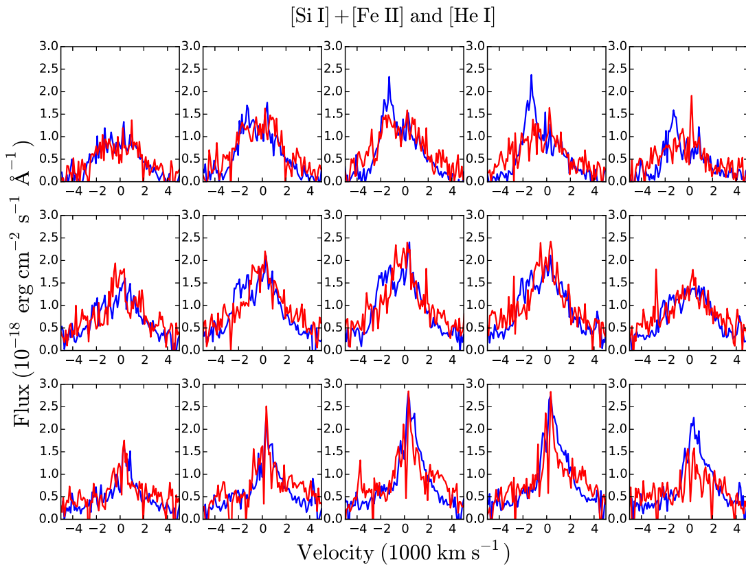
Figure 22. Comparison of the [Si I]+[Fe II] 1.644 \mu\text{m} (blue) and He I 2.058 \mu\text{m} (red) lines extracted from the regions shown in Figure 8. The He I lines have been multiplied by a factor of two.
