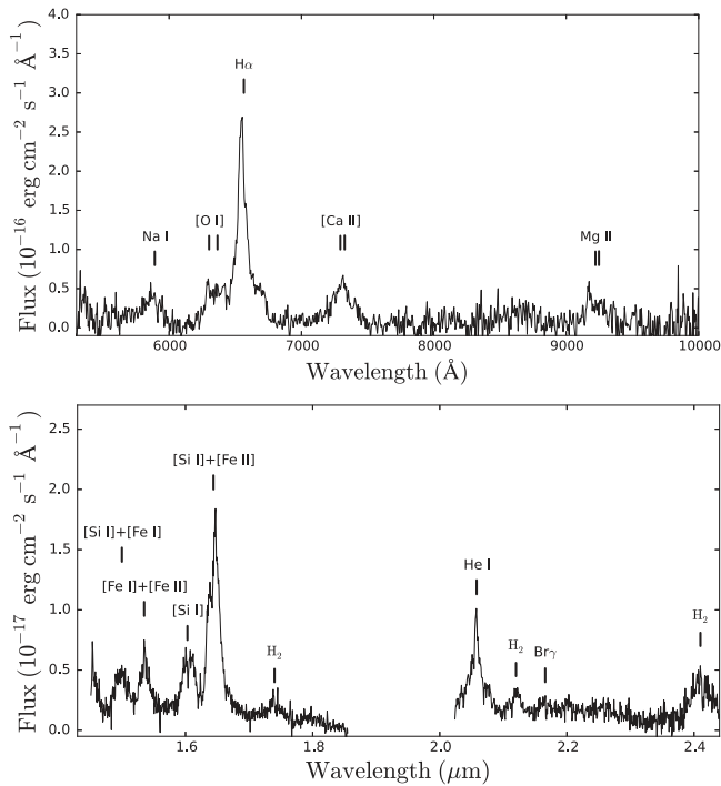
Figure 3. Upper panel: total STIS G750L spectrum of the ejecta obtained by summing all five slits. The extraction region is indicated in Figure 2. The spectrum has been corrected for scattered light from the ring. Lower panel: total ejecta spectrum in the SINFONI H and K bands. The data have been binned by a factor of three and corrected for scattered light from the ring.
