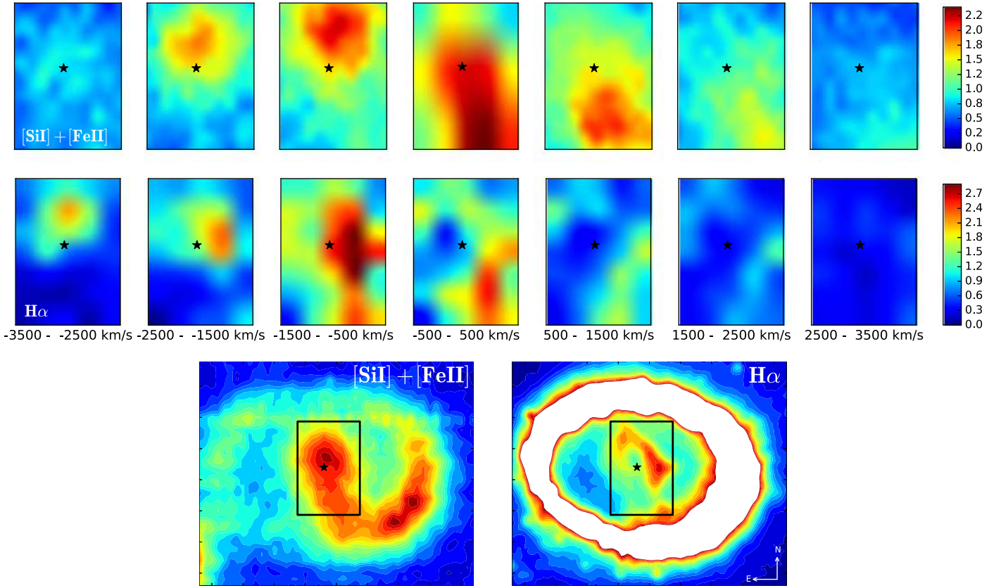
Figure 9. Images of the ejecta in velocity slices for [Si I]+[Fe II] (top row) and H\alpha (middle row), smoothed with a 2D spline function. The color bars show the intensity in units of 10^{-17} erg \text{cm}^{-2} \text{s}^{-1} and 10^{-16} erg \text{cm}^{-2} \text{s}^{-1} , respectively. The plotted regions are indicated by the black boxes in the bottom row on the contour plots for the SINFONI [Si I]+[Fe II] 1.644 \mu\text{m} , \pm 3000 \text{km s}^{-1} image (left) and the WFC3/F625W image (right). Both data sets have been corrected for emission from the ring. In the case of [Si I]+[Fe II], this results in a significantly lower spatial resolution in the central bin (see text for details). Taking the center of the ring (black star) as the point of zero velocity, the plotted area covers [-2000, +2300] \text{km s}^{-1} in the x -direction and [-3300, +2800] \text{km s}^{-1} in the y -direction.
