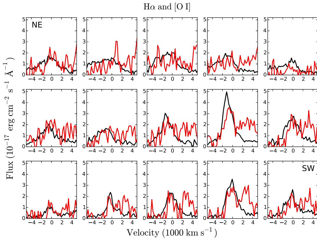
Figure 16. Comparison of the H\alpha (black) and [O I] \lambda\lambda 6300, 6364 (red) lines extracted from the regions shown in Figure 8. For [O I] the spectrum has been multiplied by a factor of four and centered on zero velocity for the 6300 Å component. The two components are separated by about 3000 \text{ km s}^{-1} .
