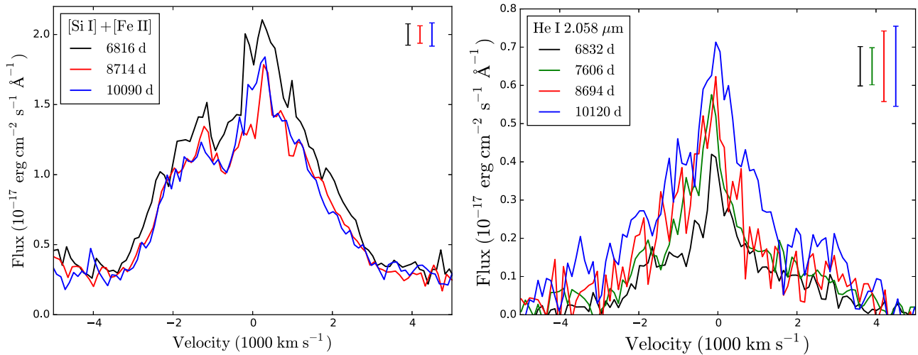
Figure 14. Comparison of line profiles from the full ejecta. Left: evolution of the [Si I]+[Fe II] 1.644 \mu\text{m} line. Right: evolution of the He I 2.058 \mu\text{m} line. All spectra have been binned by a factor of three and corrected for scattered light from the ring. For the He I line the continuum level has also been subtracted (see text for details). Error bars corresponding to the 1\sigma statistical error for the different spectra are shown in the upper right corners.
