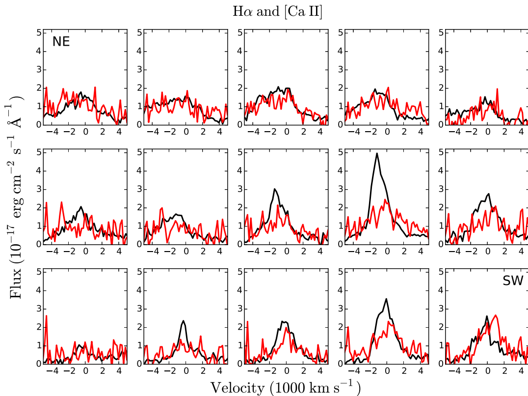
Figure 18. Comparison of the H\alpha (black) and [Ca II] \lambda\lambda 7292, 7324 (red) lines extracted from the regions shown in Figure 8. For [Ca II] the spectrum has been multiplied by a factor of three and centered on zero velocity for the average wavelength of the two components. The velocity difference between the two components is about 1300 \text{ km s}^{-1} .
