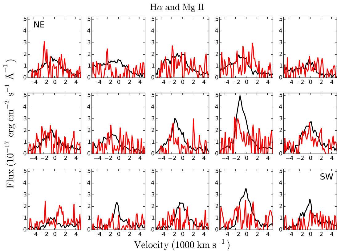
Figure 20. Comparison of the H \alpha (black) and Mg II \lambda\lambda 9218, 9244 (red) lines extracted from the regions shown in Figure 8. For Mg II the spectrum has been multiplied by a factor of four and centered at 9226\text{\AA} based on the statistical weight of the two components.
