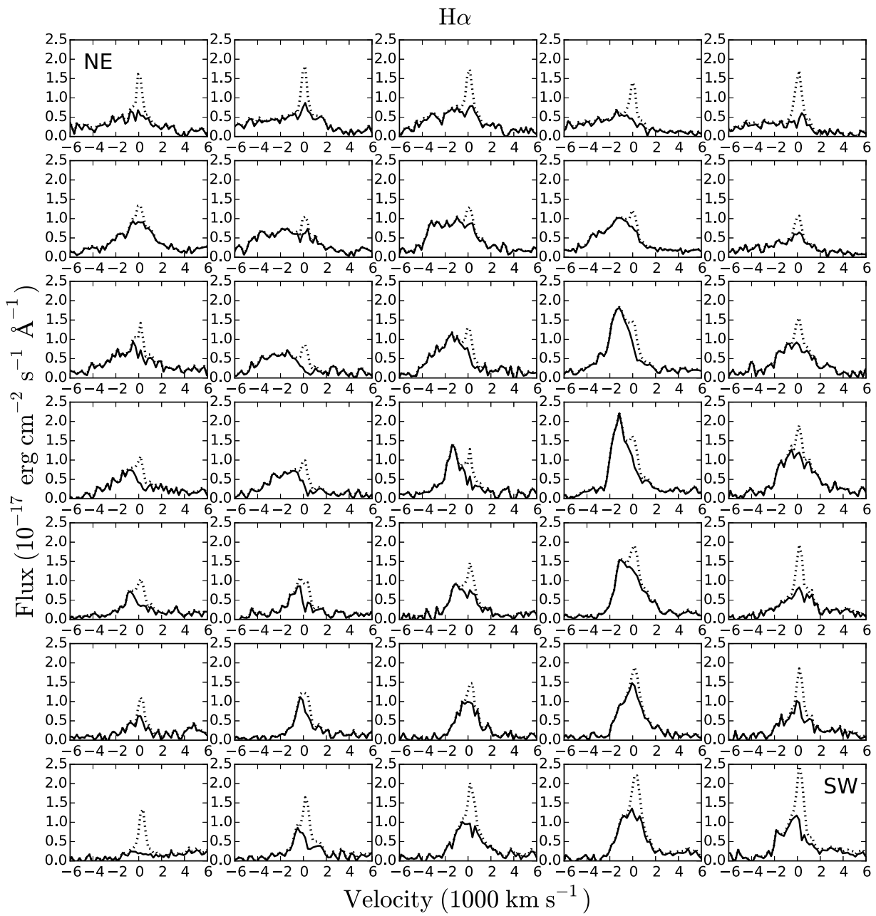
Figure 6. Spatially resolved STIS G750L spectra of H\alpha , extracted from 0''.1 \times 0''.1 regions of the ejecta. The regions are shown superposed on the WFC3/F625W image in the bottom panel. The panels with the line profiles are organized in the same way as the regions, with the upper left panel corresponding to the region in the northeast corner. At this epoch 0''.1 corresponds to 866 \text{ km s}^{-1} . The dashed and solid lines show the spectra before and after correcting for scattered light from the ring, respectively.
