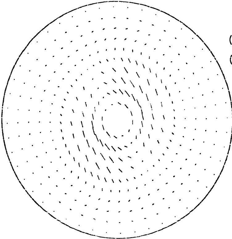
Momentum Density ( \text{g}/\text{cm}^2\text{s} ) Rotating Frame FIGURE 116
