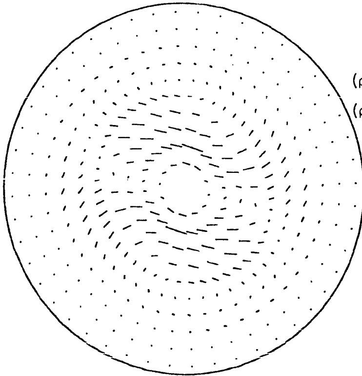
Momentum Density ( \text{g}/\text{cm}^2\text{s} ) Rotating Frame FIGURE 103
