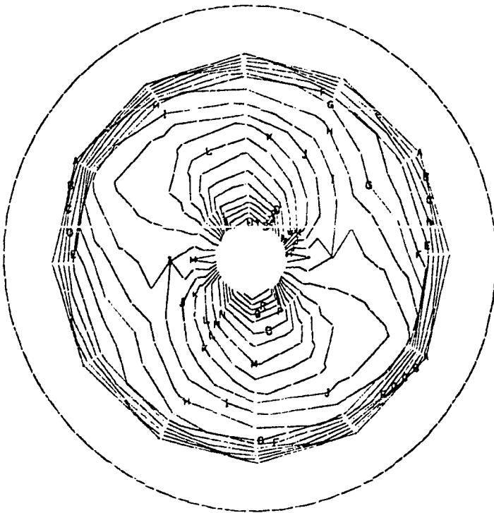
Angular Velocity( s^{-1} ) FIGURE 85
