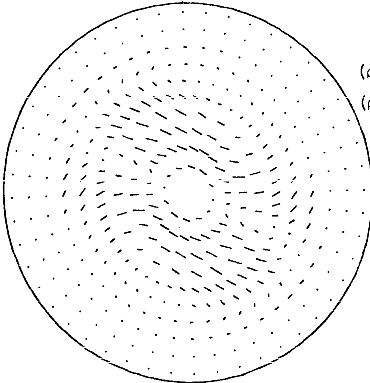
Momentum Density ( \text{g}/\text{cm}^2\text{s} ) Rotating Frame FIGURE 104
