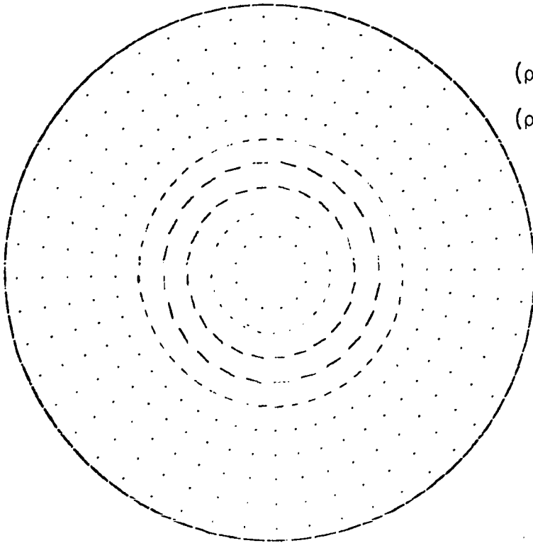
t = 0 Laboratory Frame FIGURE 54
