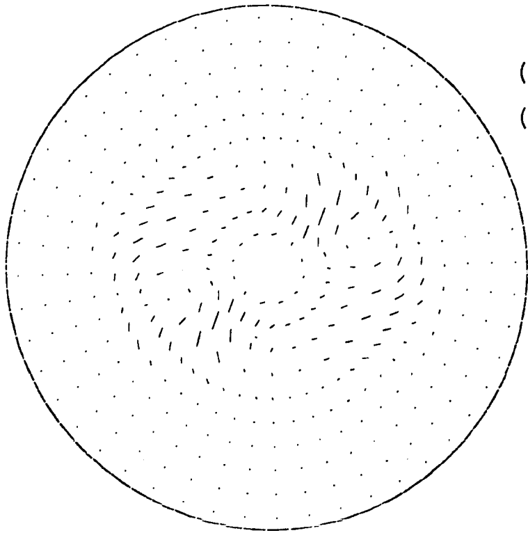
Momentum Density ( \text{g/cm}^2\text{s} ) Rotating Frame FIGURE 59
