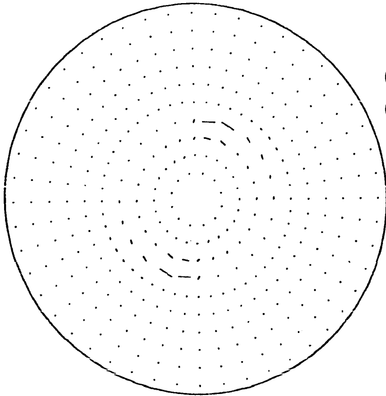
Momentum Density ( \text{g/cm}^2\text{s} ) Rotating Frame FIGURE 46
