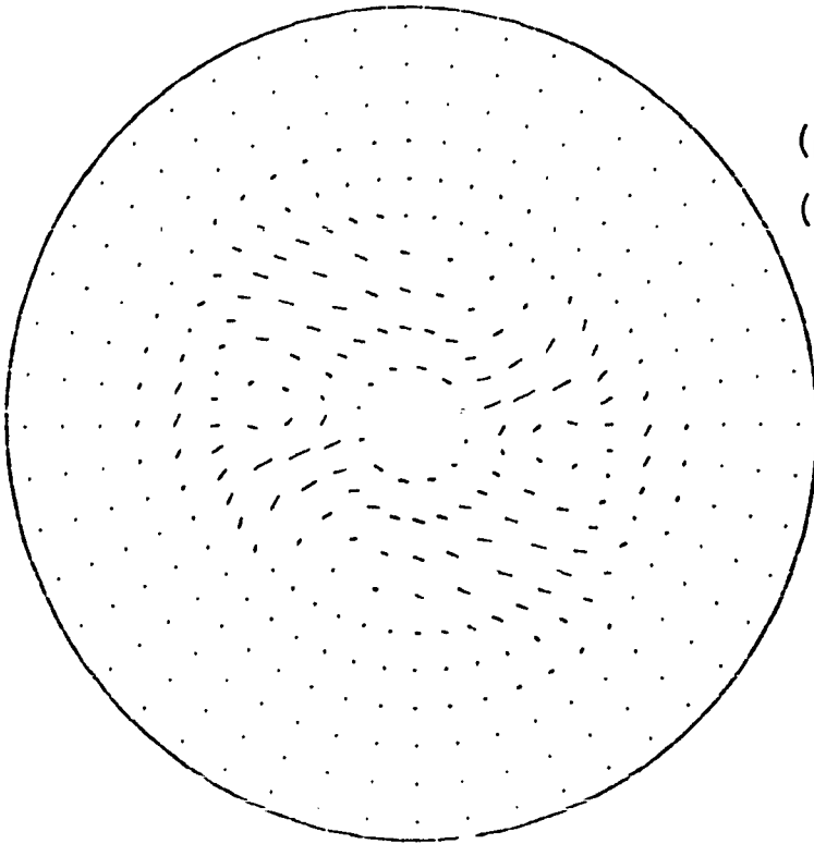
Momentum Density ( \text{g}/\text{cm}^2\text{s} ) Rotating Frame FIGURE 73
