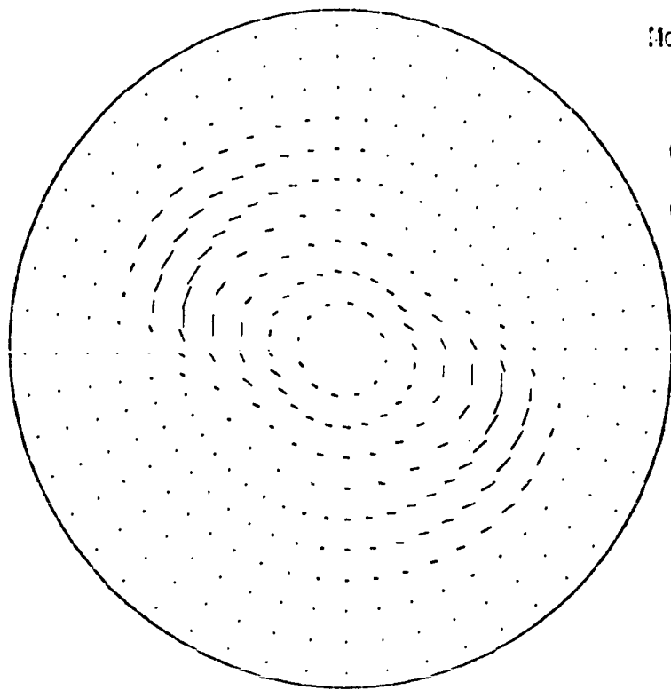
t = 1.77 \times 10^5 yrs Laboratory Frame FIGURE 77
