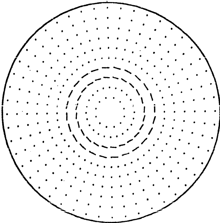
t = 0 Laboratory Frame FIGURE 41
