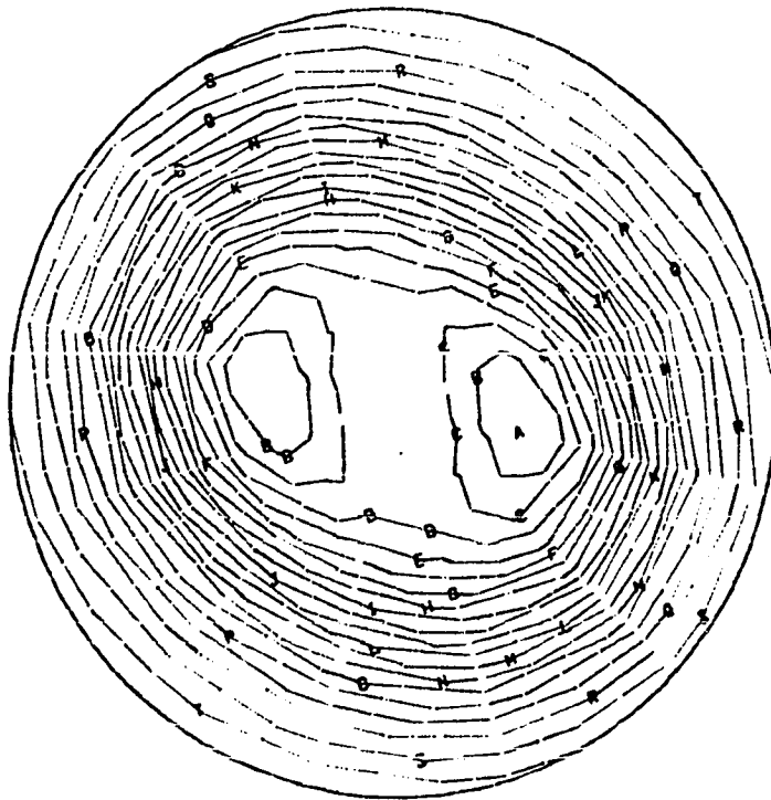
Gravitational Potential(ergs/g) FIGURE 99
