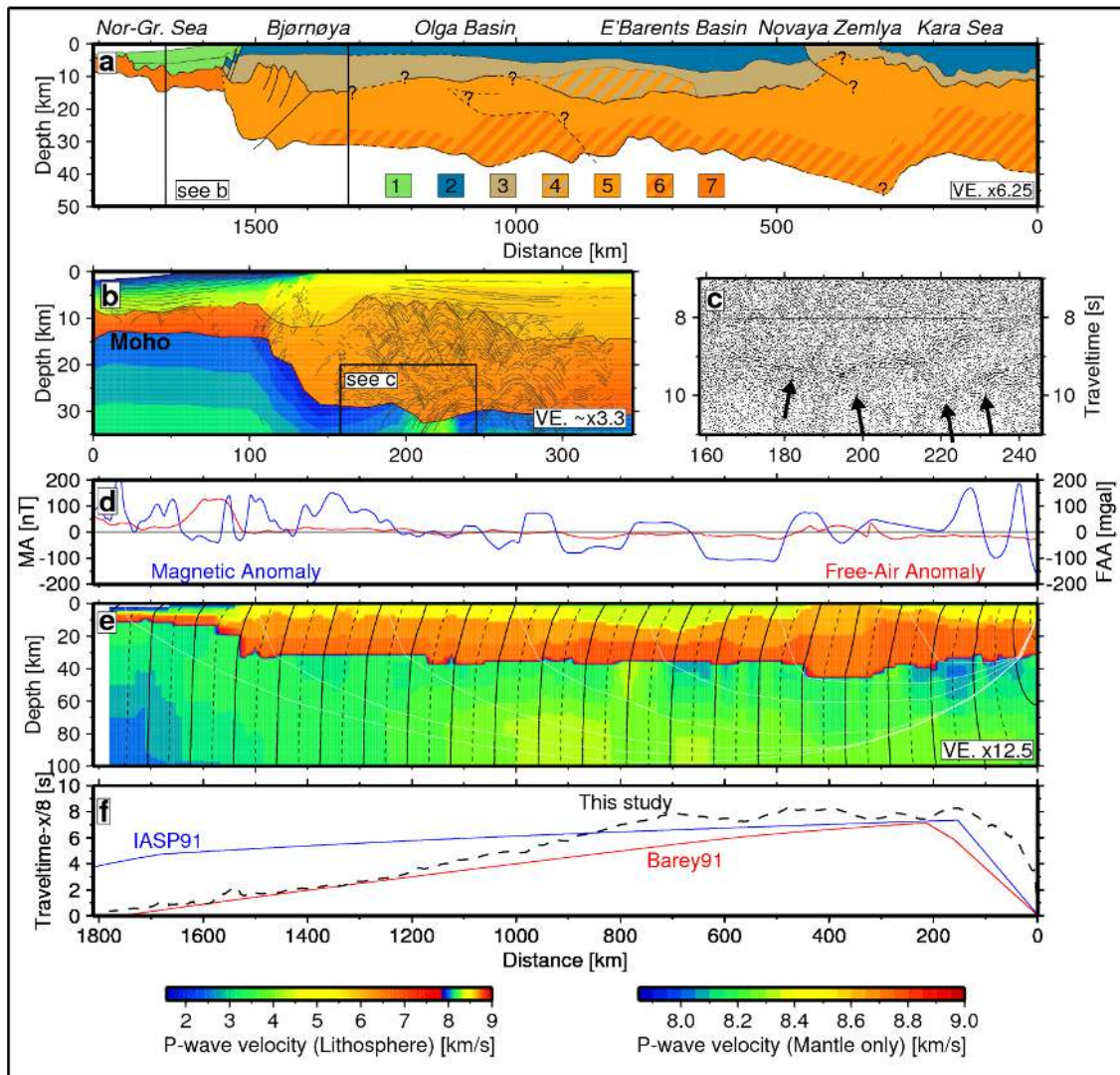
Figure 2: Observations, interpretations, and modeling for the Barents Sea A–A' transect shown in Figure 1. Figure 2a shows the geological units along the transect ranging from the oceanic crustal domain in the very west to Novaya Zemlya and the Kara Sea in the east. Along the 1800-km-long transect, all available data were used to display the distribution of sedimentary and crystalline crustal rocks: 1, Cenozoic sediments; 2, Mesozoic sediments; 3, Paleozoic sediments; 4, Paleozoic sediments and/or crystalline rocks; 5, continental crystalline rocks; 6, lower crustal crystalline rocks with V_p 6.6–6.8 km/s; and 7, oceanic crystalline rocks. Figures 2b and 2c illustrate database examples along this transect, i.e., a P-wave velocity model (with line drawing) and deep seismic reflection data, respectively (see insert boxes for along-transect location). Figure 2d shows potential-field data along the profile, Figure 2e shows the 3-D model with superimposed seismic wave fronts, and Figure 2f shows travel times in comparison with two 1-D models. For the velocity models in Figures 2b and 2e the lower color scales apply, where the left scale covers the entire range of lithospheric velocities and the right scale covers the mantle velocities only. Note that at 7.8 km/s the scale shows repeating colors (crust-mantle transition).
