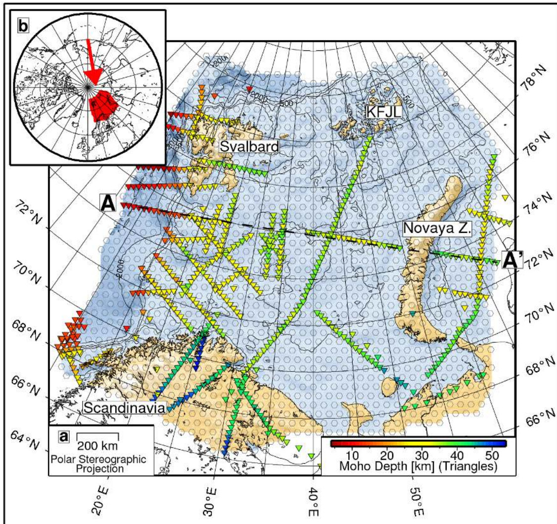
Figure 1: Map of the greater Barents Sea region, shown in red in the inset map. The lines marked with triangles are wide-angle profiles where the color coding indicates the Moho depth. The small hexagons are tiles spaced 50 km apart that will be filled with crustal and upper mantle velocities. The profile A–A is the one for which detailed results are shown in Figure 2. KFJL, Kaiser Franz Josef Land.
