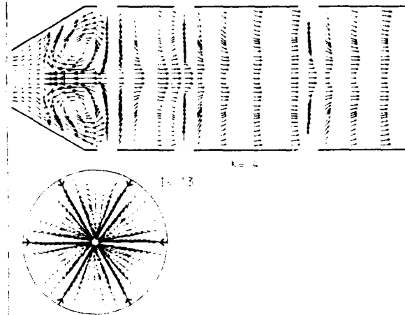
Fig.3. Velocity vectors in the hot reacting flow
