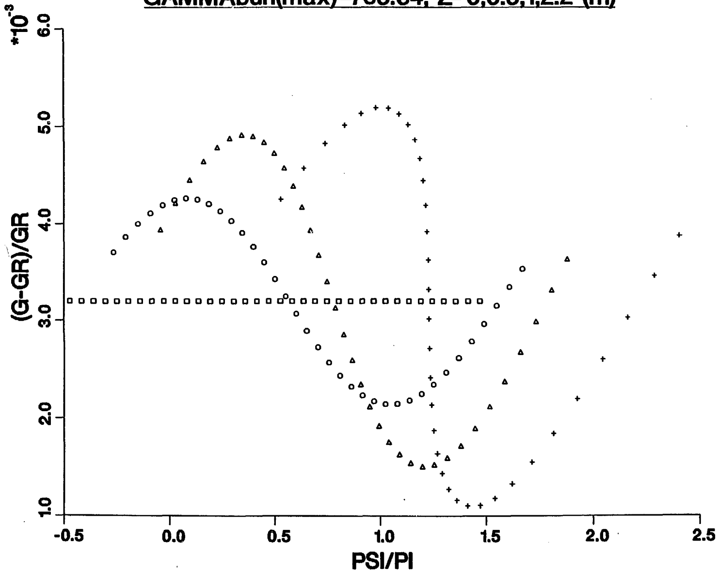
Fig. 3 Energy-phase-space diagram of electrons at four different points along the wiggler for beam energy tuning to maximum phase bunching \gamma = \gamma_{bunch}^{max} .
