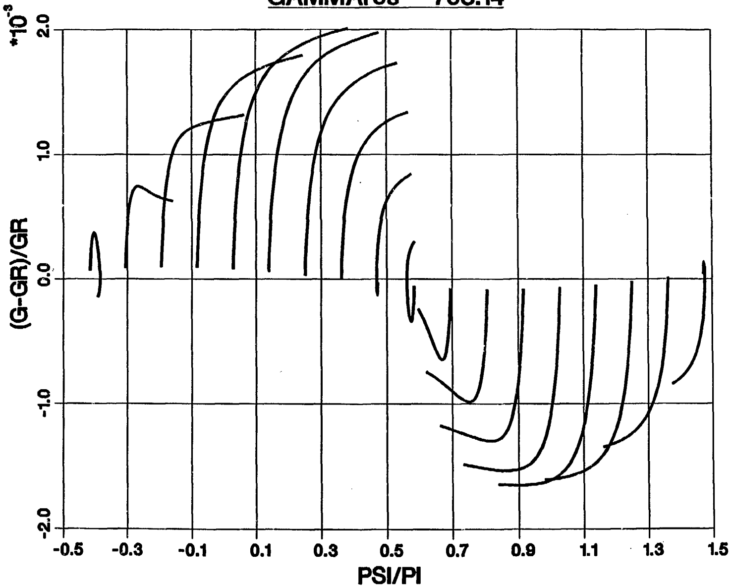
Fig. 4 Continuous Energy-phase-space diagrams of electron trajectories along the entire wiggler for beam energy tuning to plan wave resonance condition \gamma = \gamma_R .
