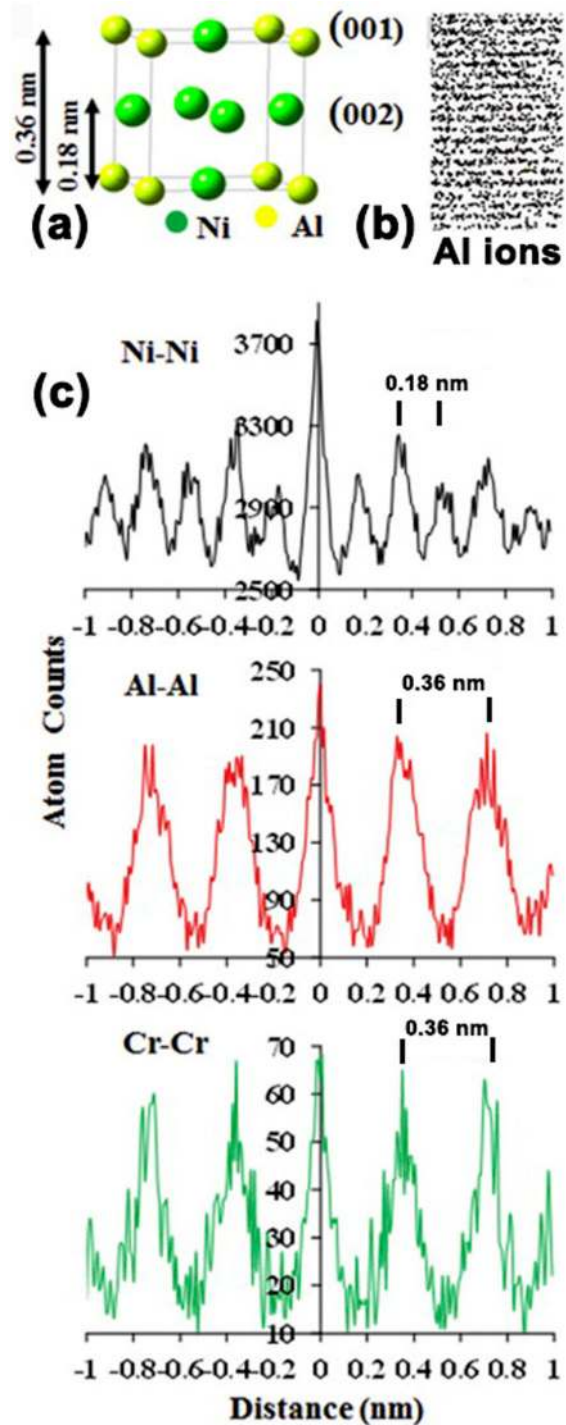
Figure 17. Ordering and site occupancy in \text{Ni}_3\text{Al} revealed by z-spatial distribution maps (adapted from Meher et al. ) [157].
