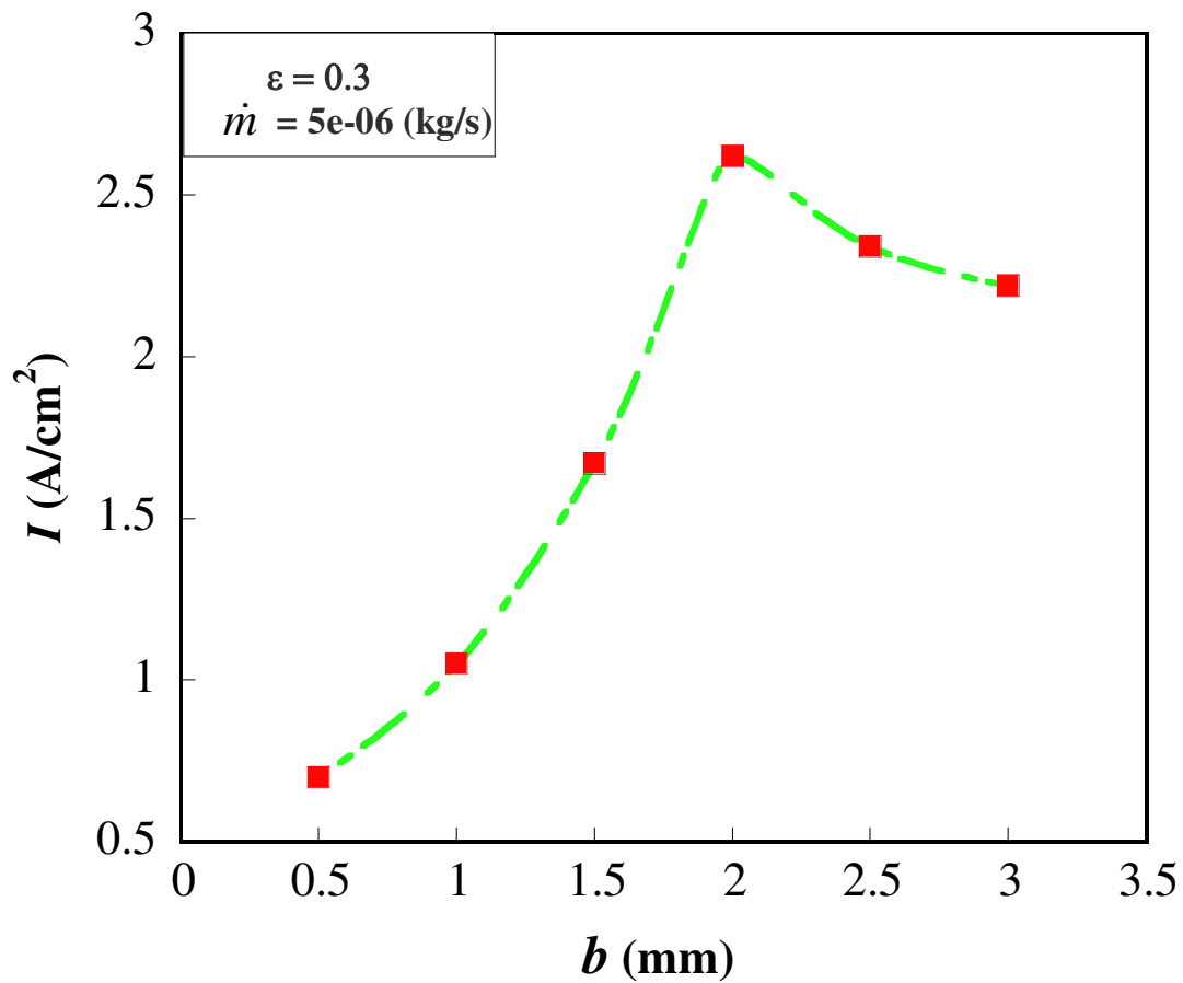
Figure 9 The cell current density at different channel depths at a cell potential of 0.3 V and a temperature 70 0 C, and a mass flow rate of 5e-06 kg/s.
