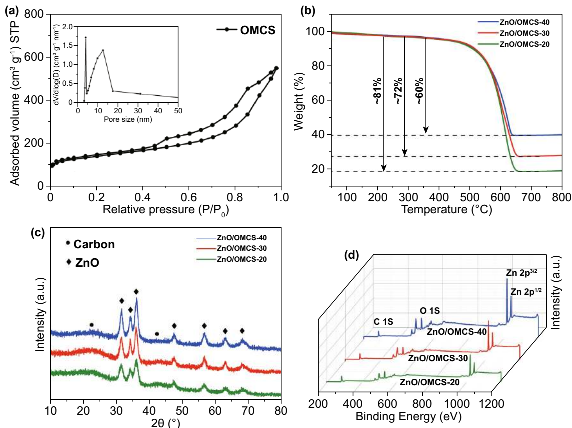
Fig. 3 a \text{N}_2 adsorption–desorption isotherms and pore size distribution of the OMCS. b TGA profiles, c XRD patterns, and d XPS spectra for the ZnO/OMCS-20, ZnO/OMCS-30 and ZnO/OMCS-40 nanocomposites
