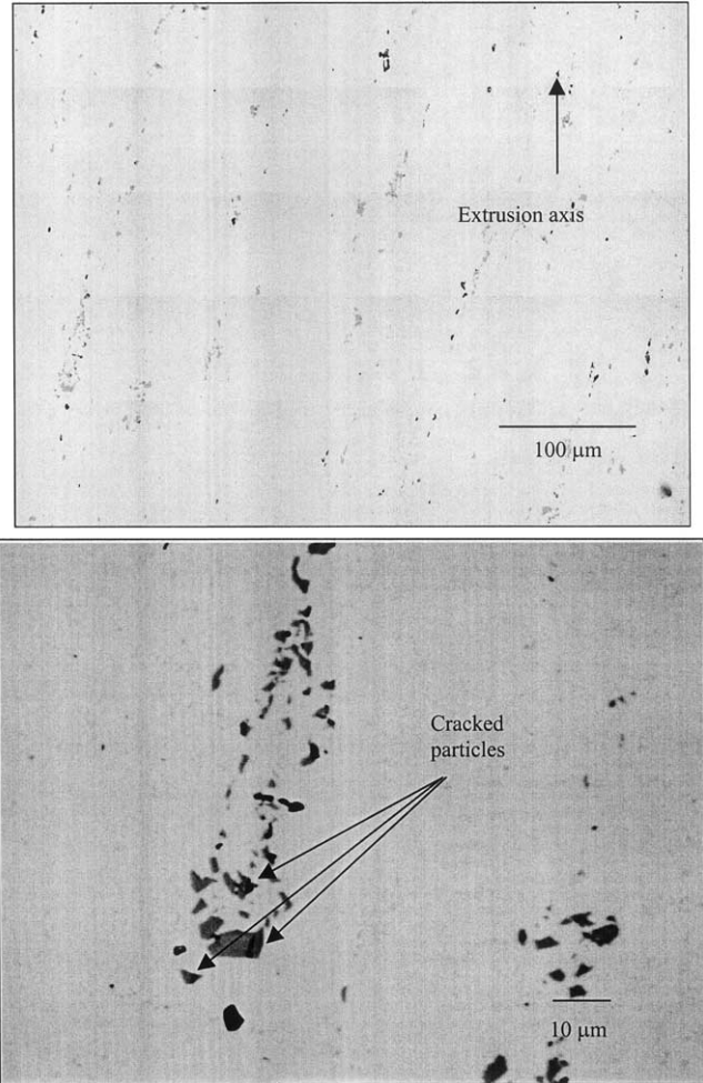
Fig. 6. Microstructure of fractured compression test specimen (0.75 strain) of 5086(O) alloy: (a) microstructural montage of 100 contiguous fields and (b) one field of view from the montage in (a) shown at the resolution level at which the montage was created. Observe that the particle cracks are mostly parallel to the extrusion axis, which is also the loading direction.
