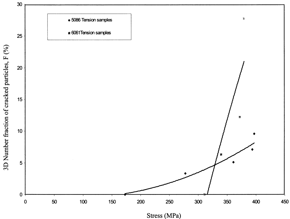
Fig. 15. Variation of 3-D number fraction of cracked Fe-rich intermetallic particles with applied true tensile stress in 5086 and 6061 Al-alloys.
