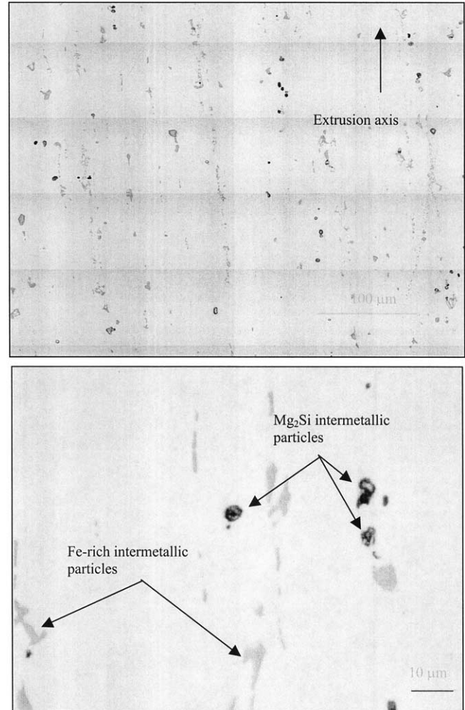
Fig. 4. Microstructure of an unstrained specimen of 6061(T6) alloy in unetched condition: (a) microstructural montage of 100 contiguous fields and (b) one field of view from the montage in (a) shown at the resolution level at which the montage was created.
