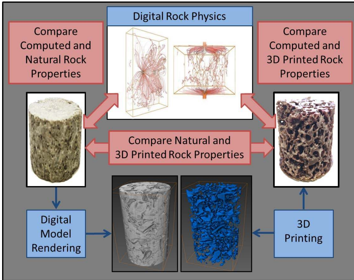
Figure 3. Workflow for comparison of macroscopic rock properties to digital models and 3D printed rock proxy properties. Macroscopic properties are defined by bulk measurements that represent a spatially averaged quantity beyond the microscopic scale and include, but are not limited to, flow (e.g., relative permeability), electrical (e.g., resistivity), acoustic (e.g., P and S wave velocities), and magnetic (e.g., NMR) properties.
