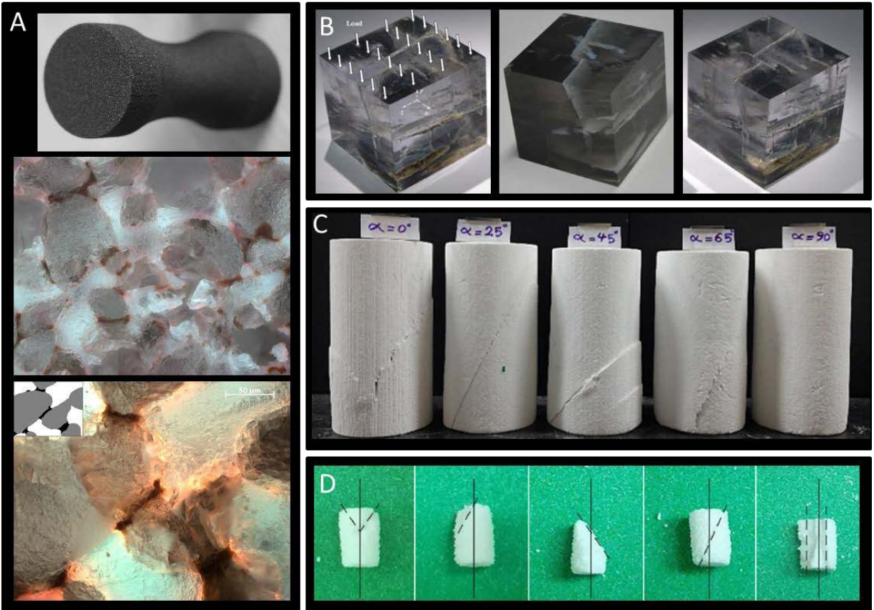
Figure 4. Applications of 3D printing to geomechanical experiments. (A) Osinga et al. (2015) manufactured proxies for uniaxial compression testing using a sand-binding 3D printer. (B) Ju et al. (2014) used 3D printing to visualize fracture geometries and associated stress concentrations in naturally occurring coal. (C) Fereshtenejad and Song (2016) tested uniaxial mechanical strength of rock proxies printed in gypsum powder. (D) Vlasea et al. (2015) explored the impact of layer orientation relative to compression direction on sample strength.
