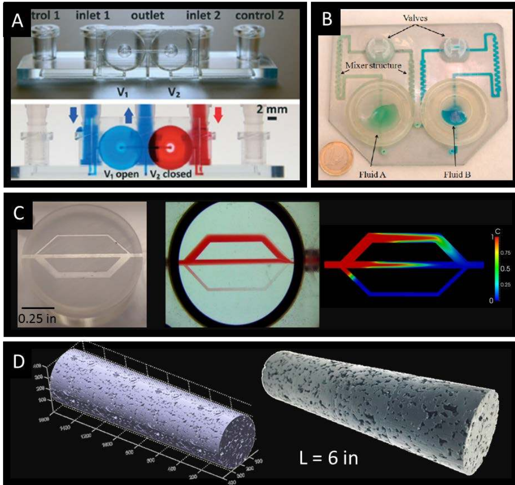
Figure 2. Selected examples of published studies using 3D printed devices and rock proxies for microfluidic and flow phenomena. (A) Yazdi et al. (2016) and (B) Bonyar et al. (2010) both show examples of translucent microfluidic devices designed for fluid mixing and homogenization for visualizing sample and reagent interactions. (C) Watson et al. (2016) demonstrated the utility of translucent 3D printed microfluidic devices for comparison of flow and transport experiments with direct numerical simulations. (D) This is an example of a 3D digital representation of a natural sandstone core plug (left) and the 3D printed rock proxy used in core flood experiments (right) at the Aramco Research Center in Houston.
