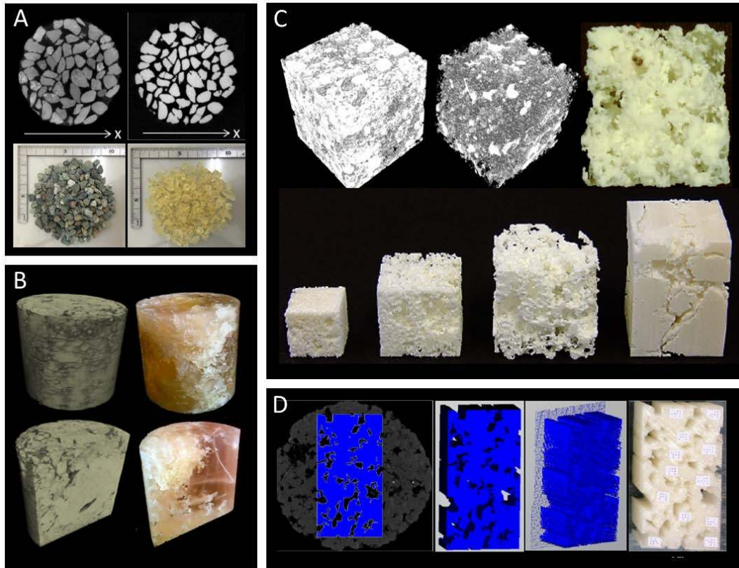
Figure 1. Selected examples of published studies using 3D printed rock proxies generated from digital models. (A) Matsumura and Mizutani (2015) 3D printed gravel material to evaluate the mechanical behavior of soil structures. Shown are X-ray micro-CT scan sections and images representing natural and 3D printed gravel. (B) Dal Ferro et al. (2015) used 3D printing to represent large undisturbed soil cores. 3D representations shown are of X-ray micro-CT scans and images of the associated 3D printed soil core. (C) Similarly, Otten et al. (2012) employed X-ray micro-tomography imaging to generate a range of 3D printed soil replicas to study soil-fungal relationships. (D) Jiang and Zhao (2015) generated 3D printed rock proxies from CAD models to study a mechanical behavior of 3D printed rock proxies.
