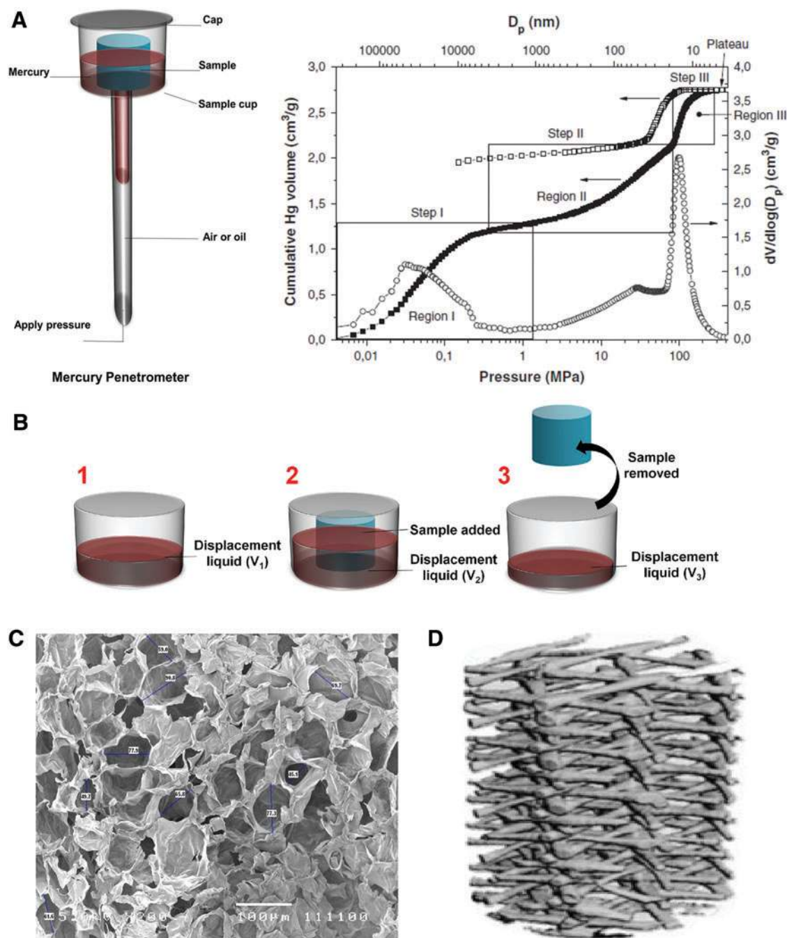
FIG. 6. Schematic illustration of (A) mercury porosimetry, (B) three-step liquid displacement process, (C) SEM imaging technique, and (D) microcomputed tomography imaging used for porosity or pore size measurement of scaffolds. Images adapted and reproduced by permission of Elsevier and IOP Publishing Ltd. (DOI: 10.1088/1758-5082/3/3/034114). 121,122 Color images available online at www.liebertpub.com/teb
