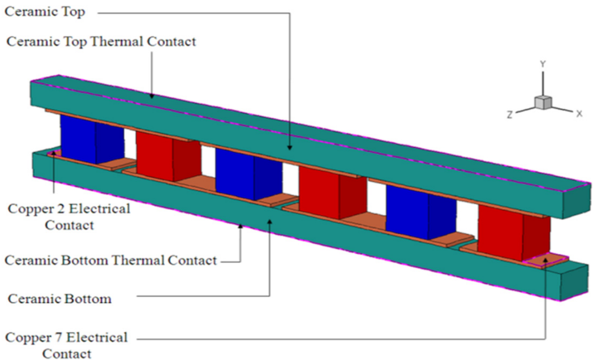
Figure 7. A 3D three couple thermoelectric module with ceramic outer plates modelled in Setaurus Structure Editor [8]
