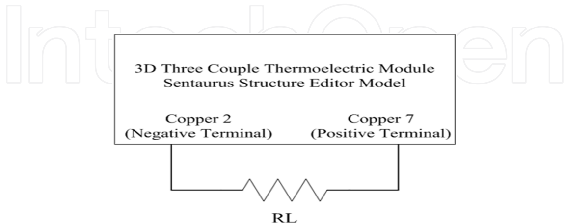
Figure 6. A schematic representation of a TCAD Mixed Mode simulation of a thermoelectric module with a load resistance RL connected between the thermoelectric model output terminals [8]
