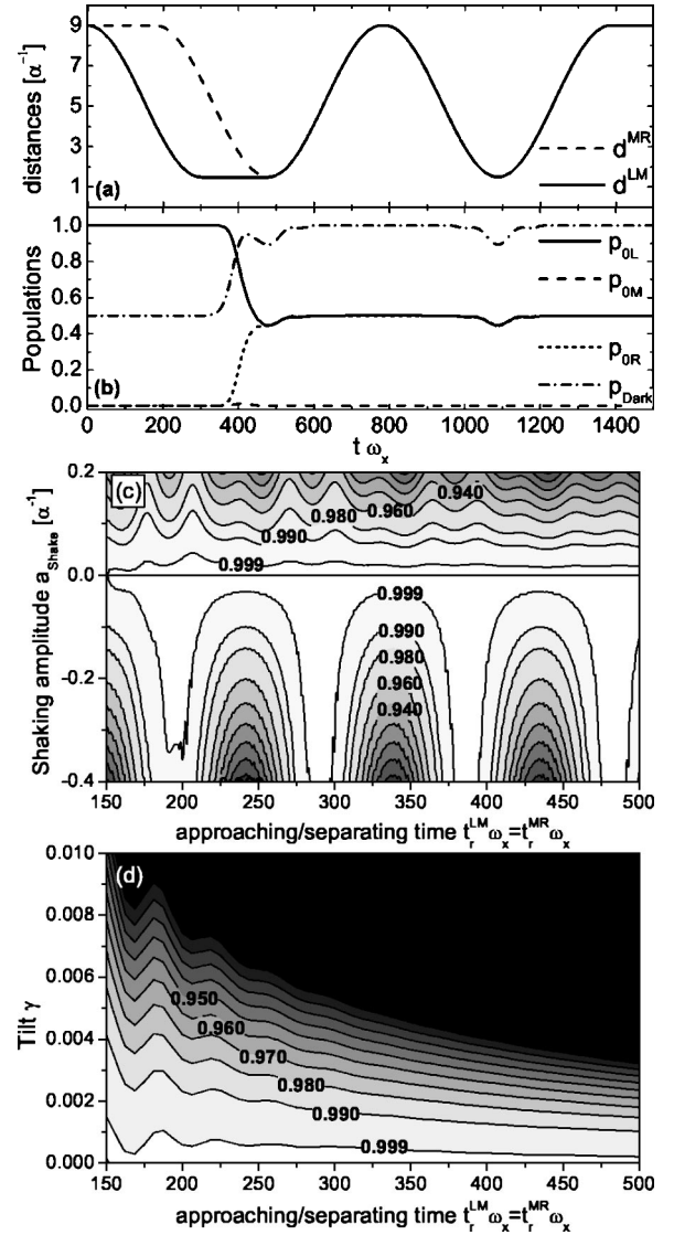
FIG. 3. (a) Approaching sequence for a CPT-like process; (b) ground state and dark state populations, p_{\text{Dark}} = |\langle D(\Theta = \pi/2) | \psi(t) \rangle|^2 ; parameters as in Fig. 2 except for t_r^{\text{LM}}\omega_x = 0 , t_r^{\text{MR}}\omega_x = t_{\text{delay}}\omega_x = 180 for t\omega_x \leq 780 and t_r^{\text{MR}}\omega_x = t_{\text{delay}}\omega_x = 0 for t\omega_x > 780 . (c) Dark state population p_{\text{Dark}} after the CPT process as a function of the time t_r used to approach and separate the traps (horizontal axis) and of the amplitude a_{\text{shake}} of a shaking in the trap positions (vertical axis). For a_{\text{shake}} > 0 , the shaking of the outer traps is in phase; for a_{\text{shake}} < 0 , it is out of phase by \pi ; \omega_{\text{shake}} = 10^{-2}\omega_x and all other parameters as above except for t_{\text{delay}} = 0.6t_r . (d) p_{\text{split}} [see Eq. (4)] for an additional tilted potential as in Fig. 2(d) parametrized by \gamma as a function of the time t_r needed to approach and separate the traps; parameters as in (c).
