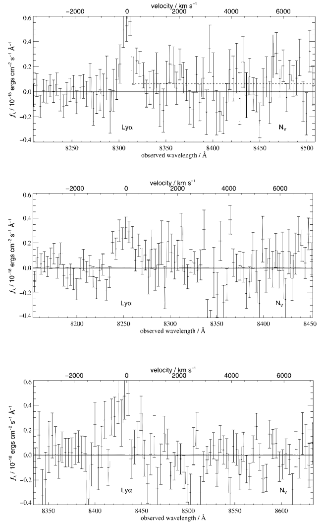
FIG. 2.—Unbinned GMOS-South spectra of GLARE 1042, GLARE 3001, and GLARE 3011 around the Ly \alpha candidate line emission. The continuum level is indicated on 1042
