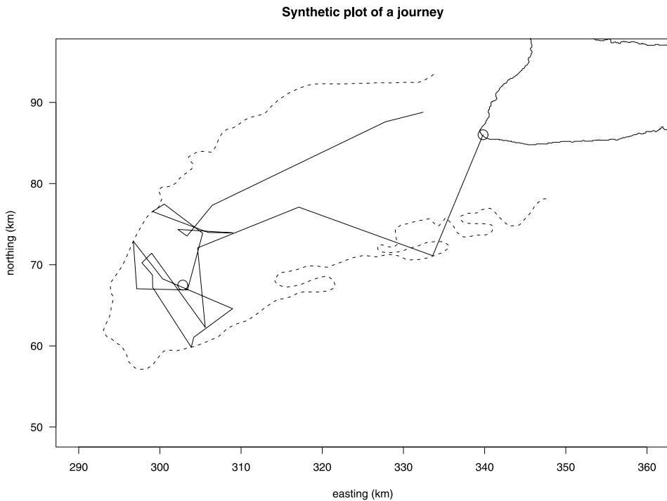
FIG 11. A simulated journey starting at La'au Point and heading towards the circle at the lower left. The potential function of Figure 9 is employed. This figure may be compared with Figure 8. The kinks in the track are the time points of journey 7 of Figure 7.
