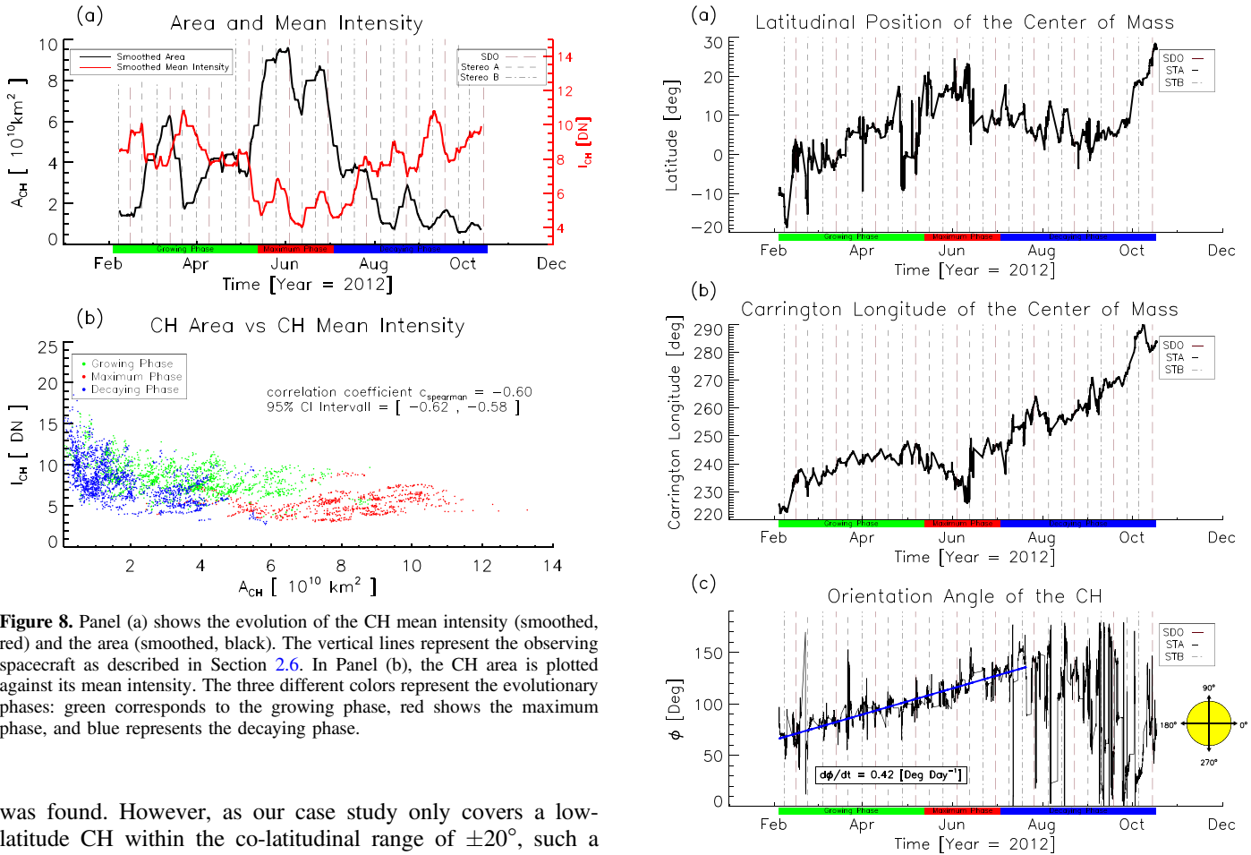
Figure 9. Motional behavior of the CH: (a) latitudinal movement of the CH; (b) longitudinal motion of the CH; (c) orientation angle of the CH together with a linear fit (blue) for the time where the angle can be derived unambiguously. The vertical lines in (a)–(c) represent the observing spacecraft as described in Section 2.6.
