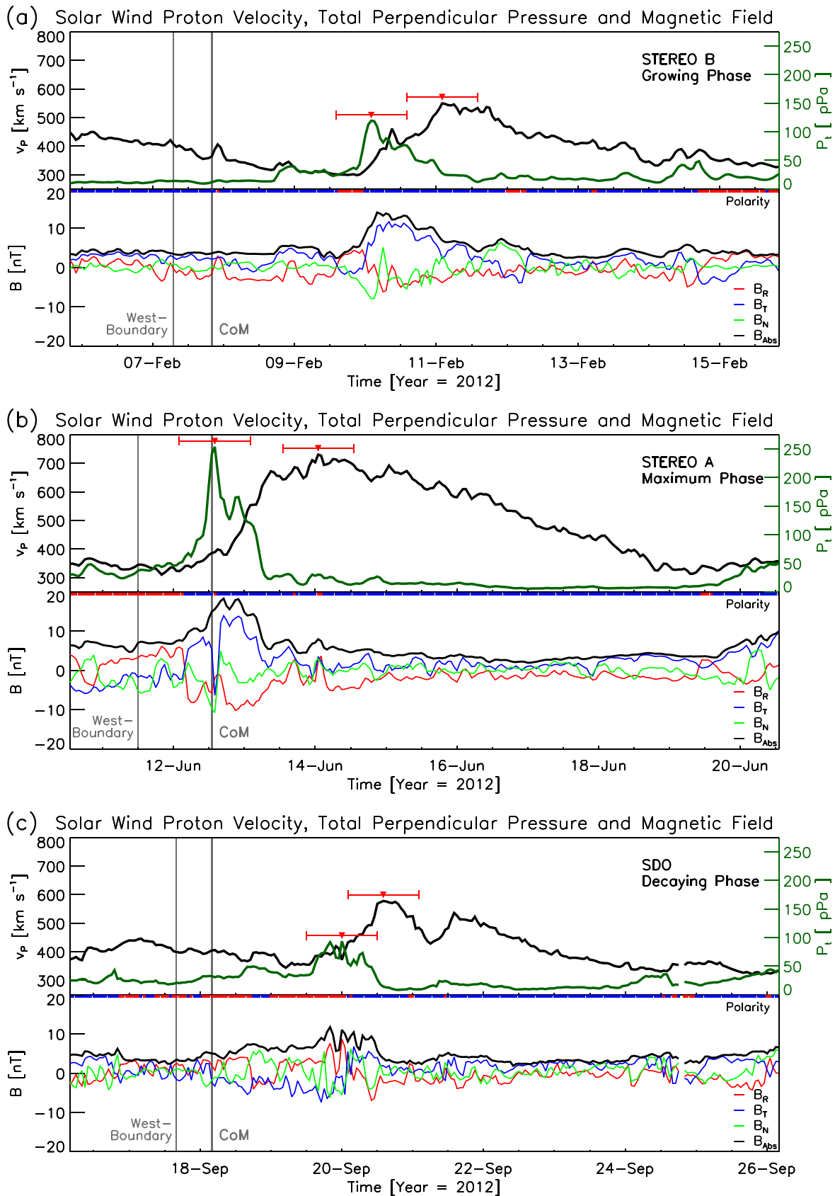
Figure 2. Examples of in situ signatures of the solar wind as observed by STEREO-B , STEREO-A , and OMNI , as the CH under study was observed near the center of the solar disk by STEREO-B , STEREO-A , and SDO , respectively. The panels (a)–(c) represent different stages in the CH evolution. The top panels show the solar wind bulk velocity (black) and total perpendicular pressure (green), and the bottom panels show the magnetic field components (RTN and absolute value). The red-blue bar below the velocity-pressure plot indicates the magnetic field polarity of the solar wind, with red representing positive and blue negative (=CH) polarity. The gray vertical lines are the time when the CH makes a CMP with the CoM and the west boundary. The red bars indicate the manually extracted peak (triangle) and the \pm 12 hr interval over which the parameter was averaged.
