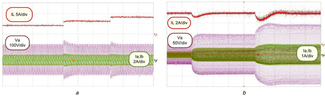
Fig. 12 Input to output decoupling
