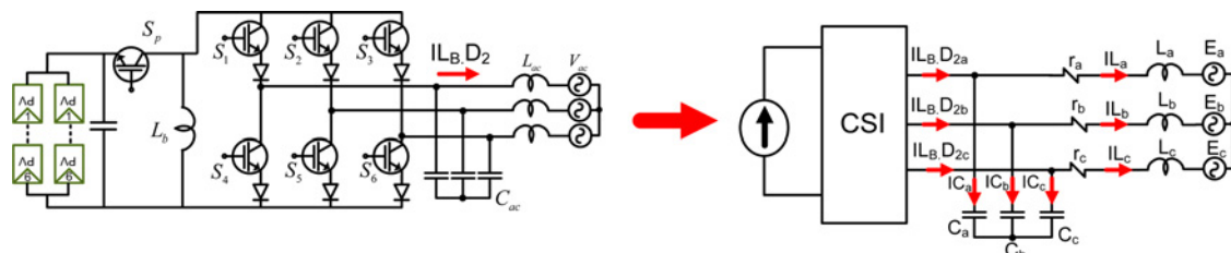
Fig. 6 Equivalent circuit for controlling the converter's output
