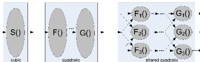
Fig. 1: Decomposition approach
