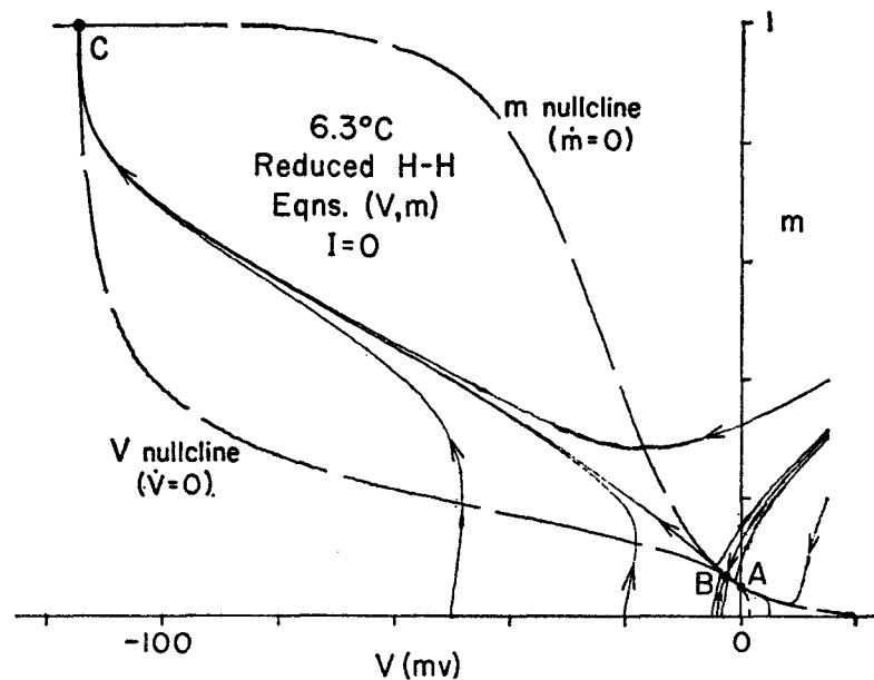
FIGURE 2. Phase plane of V, m reduced Hodgkin-Huxley system, with h and n fixed at their resting values and I = 0 . Solutions of equations follow paths marked with arrowheads. Three singular points occur at intersections of nullclines (curves on which \dot{V} = 0 and \dot{m} = 0 respectively). Threshold phenomenon appears at saddle point B . Stimulus displaces phase point from resting singular point A , and is followed by either return to A or passage to singular point C (excitation), depending on shock strength.
