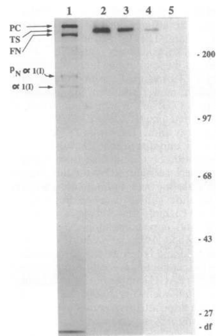
FIG. 2. TSP levels in BAEC and RVEC before and after the organization of endothelial cords. BAEC (lanes 1, 2, and 3) and RVEC (lanes 4 and 5) were metabolically labeled with [ ^3 H]proline at subconfluence (lanes 2 and 4) and after the formation of endothelial cords (lanes 1, 3, and 5). Medium was dialyzed against 0.1 M acetic acid and lyophilized. Radiolabeled proteins from 250,000 cells were subjected to electrophoresis on a nonreducing SDS/polyacrylamide gel and were visualized by autoradiography (lane 1). An identical gel was transferred to nitrocellulose and incubated with anti-TSP IgG followed by ^{125} I-labeled protein A (lanes 2–5). Immunolocalized TSP was identified by autoradiography. Globular protein standards are shown on the right in kDa. Types I and III procollagen (PC), TSP (TS), fibronectin (FN), and processed chains of type I procollagen ( P_N\alpha 1 , \alpha 1 ) have been identified. df, Dye front.
