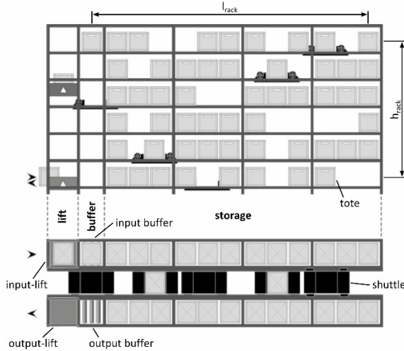
Figure 1. Shuttle system [5]
