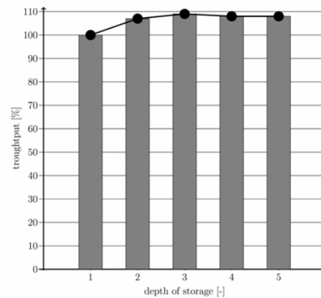
Figure 8. Throughputs of a shuttle system with optimized geometry and multi-depth storage
