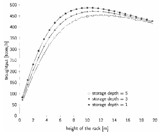
Figure 5. Throughput \vartheta_{system} of a shuttle system with multi-depth rack at 100m rack length
