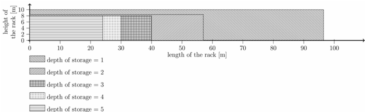
Figure 10. Dimensions of the optimized rack
