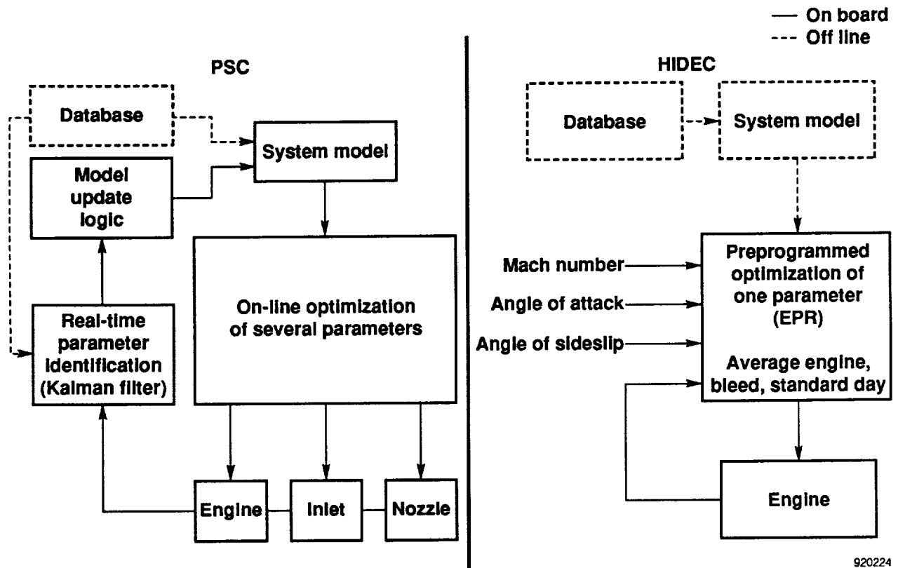
Fig. 3 Comparison of PSC and HIDEc block diagrams.
