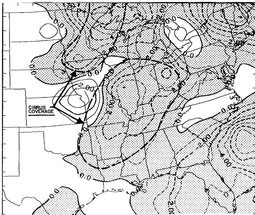
a. d\theta/dt ( ^{\circ}\text{C}/3\text{h} ) at 200 mb at 0600 GMT 25 April.
