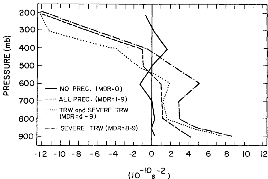
Fig. 35. Average profiles of \{k \cdot (\vec{v}_p \times \frac{d\vec{v}}{dt})\} as a function of pressure and MDR coded precipitation intensity. (Maximum MDR value was assigned to a grid point within 1/2 grid distance ( \approx 80 km) from MDR 3-h composite charts).
