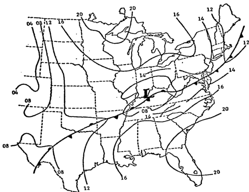
b. Surface pressure and frontal analysis
