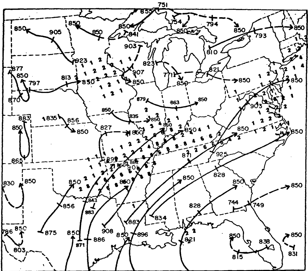
a. Parcel terminating at 850 mb. (tick marks at successive 12-h positions along the trajectories).
