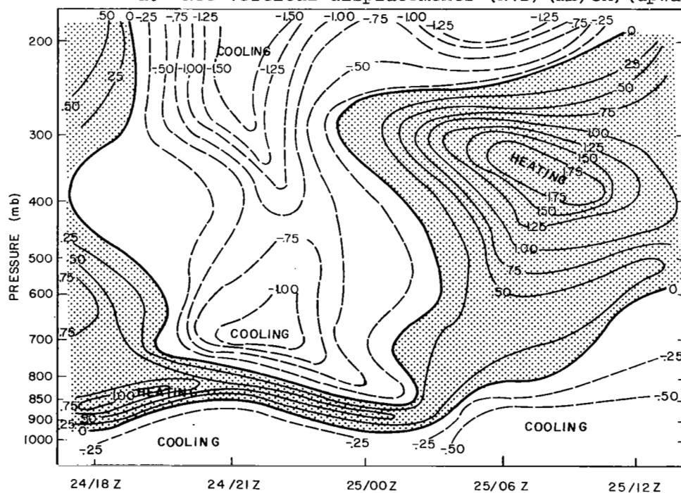
b. \frac{d\theta}{dt} ( ^{\circ}\text{C}/3\text{h} ) (heating shaded).
