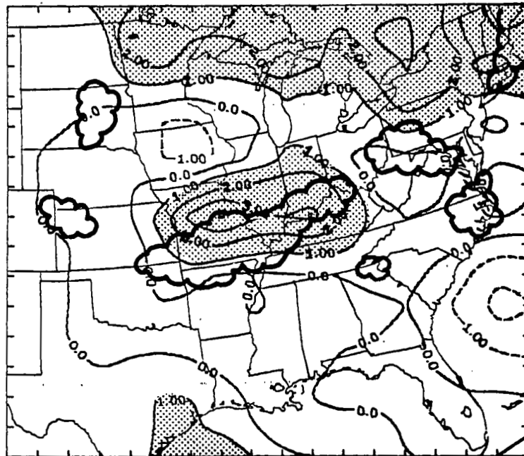
1200 GMT, 24 April c. 300 mb
