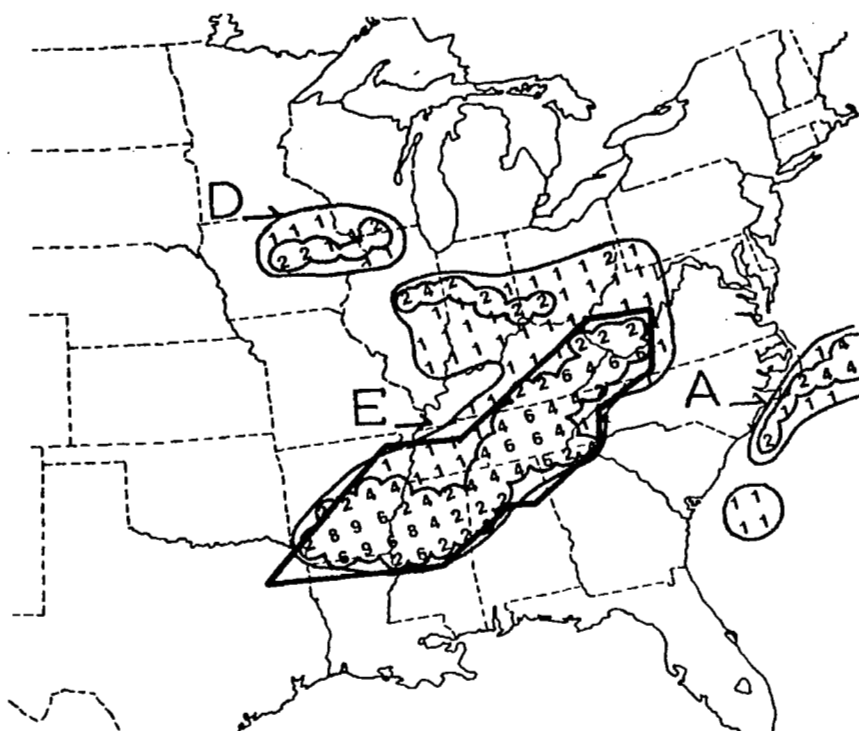
a. Composite MDR precipitation analysis
