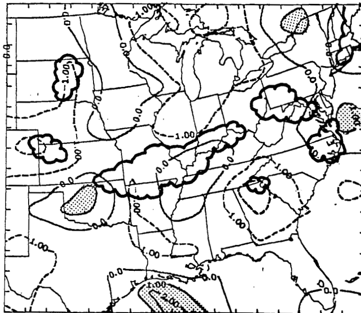
Fig. 26. Spatial fields of \frac{d\theta}{dt} ( ^{\circ}\text{C}/3\text{h} ) for the first two analyzed time periods of AVE IV at a) 900 mb, b) 600 mb, and c) 300 mb. Shaded areas are \frac{d\theta}{dt} > 1.0^{\circ}\text{C}/3\text{h} and scalloped areas are regions of convective activity.
