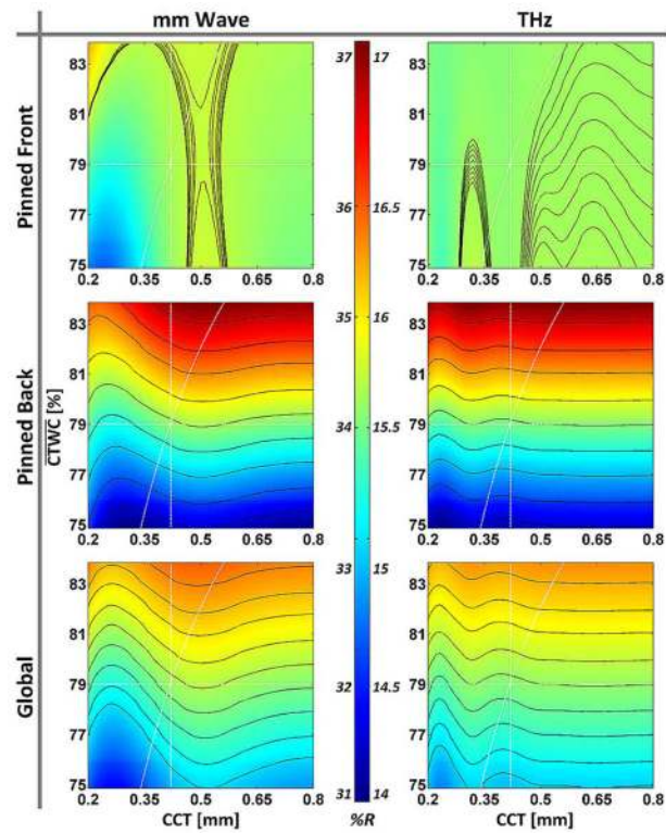
Fig. 11. Dependence of corneal reflectivity on TWC and thickness computed for the (left column) 100 GHz system and (right column) 525 GHz system for the gradient types (top row) pinned front, (middle row) pinned back, and (bottom row) global. The figures within each row are displayed with a common colormap, with pixel intensities representing reflectivity.
