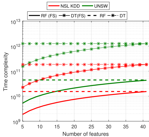
FIGURE 10. Time complexity.
