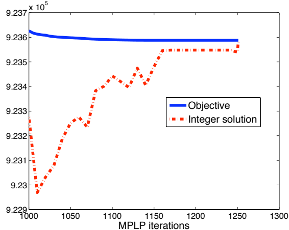
Figure 3: Dual objective and value of decoded integer solution for one of the reduced “Tsukuba” stereo models, as a function of MPLP iterations. It can be seen that both curves converge to the same value, indicating that the MAP solution was found.
