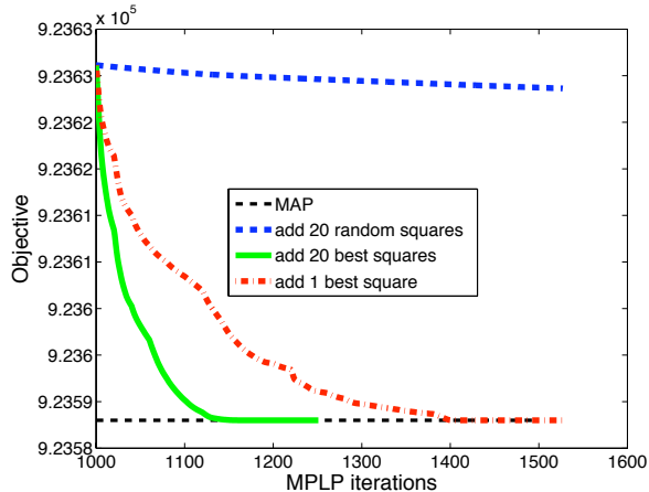
Figure 4: Comparison of different schedules for adding squares in one of the stereo problems.
