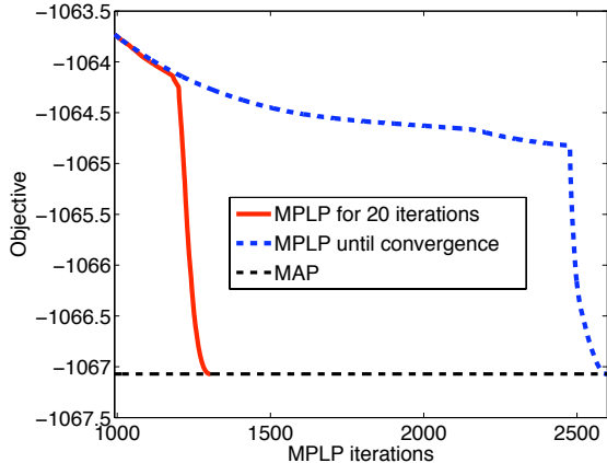
Figure 2: Comparison of different schedules for adding clusters to relaxation on a side-chain prediction problem.
