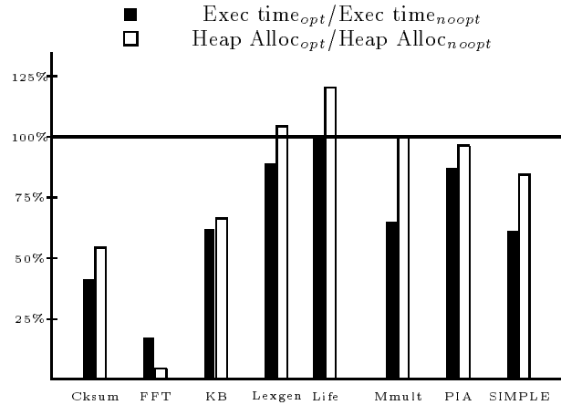
Figure 12: Effects of Loop Optimizations
