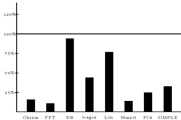
Figure 8: TIL Execution Time Relative to SML/NJ
