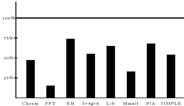
Figure 10: TIL Physical Memory Used Relative to SML/NJ
