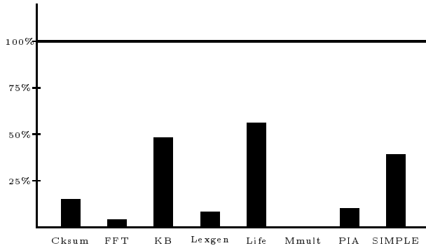
Figure 9: TIL Heap Allocation Relative to SML/NJ
