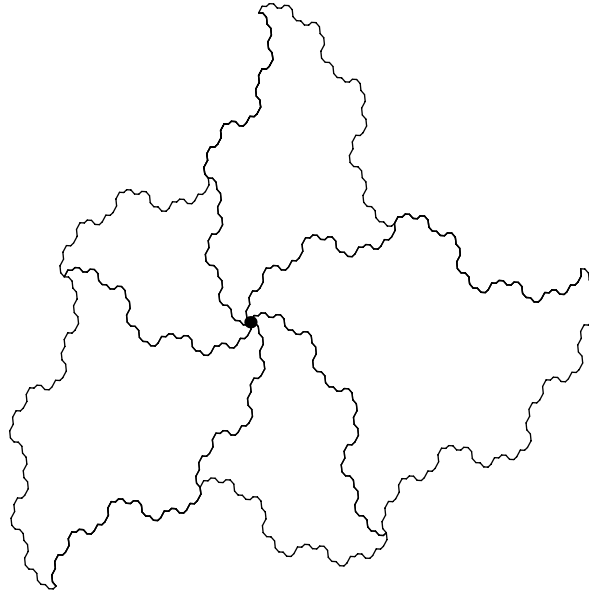
Fig. 10: The exchange of pieces: the image
