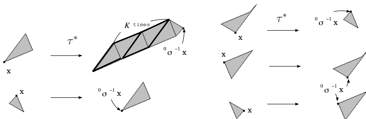
Fig. 8: The substitution \tau^*
