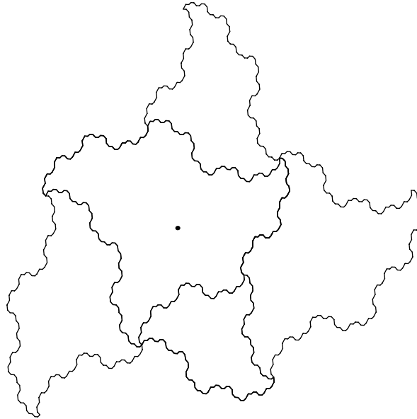
Fig. 9: The exchange of pieces: the domain
