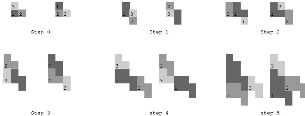
Fig. 3: Five steps of exduction
