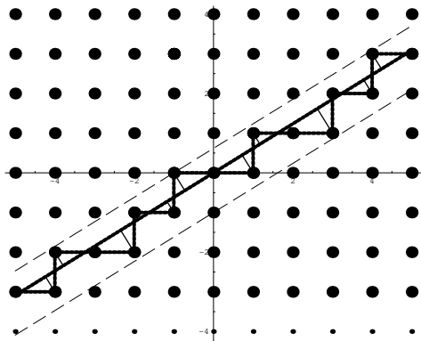
Fig. 1: The Fibonacci tiling by the “cut and project” method
