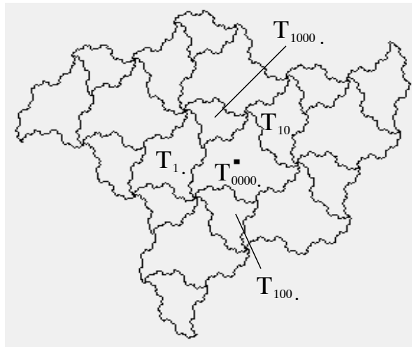
Fig. 7: The TA-tile associated with \beta
