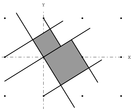
Fig. 2: The space of tilings generated by the Fibonacci tiling
