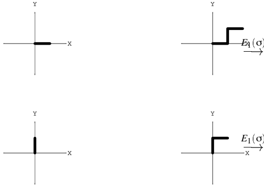
Fig. 6: The linear map associated with \mathbf{1} \mapsto \mathbf{121} , \mathbf{2} \mapsto \mathbf{21}
