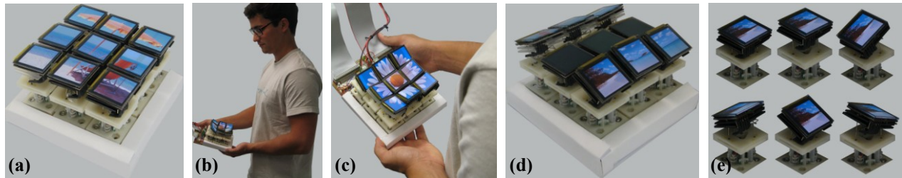
Figure 1. Tilt Displays. (a) Flat screen configuration; (b, c) User holding 12cm×12cm portable prototype; (d) Collaboration Mode; (e) Individual modules in (clockwise from top left) down, up, tilt left, tilt right, tilt forwards and tilt backwards configurations.
