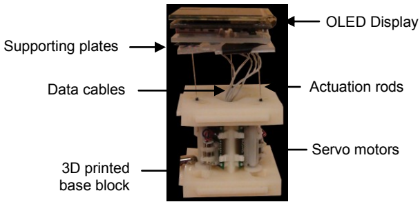
Figure 2: Prototype construction
