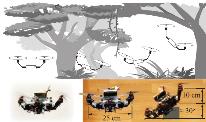
Fig. 1. The TiltDrone prototype in tilted horizontal, level, and tilted hovering flight (bottom left to right). The morphing TiltDrone can tilt up to 30 degrees, allowing it to traverse narrow areas such as dense foliage in forest environments (top).
